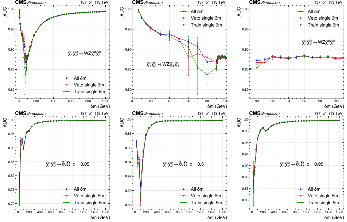
Figure 4. The AUC performance of the parametric neural networks for discriminating the signal from the total background predicted in simulation, as a function of \delta m for the trainings targeting different signal models. The top row corresponds to the neutral network targeting signals with WZ-mediated decays with different mass ranges to show all points. The bottom row corresponds to the models with slepton-mediated decays at x = 0.05 (left), x = 0.5 (middle) and x = 0.95 (right). Neural network models shown in blue are trained using all available \delta m points, those in red are trained with all available points except the point for which the performance is shown. The models in green are not parametric and only trained to find a signal at the point where the performance is indicated. Each neural network is retrained ten times, and the mean performances are shown, with error bars indicating the standard deviation computed from ten performance values. This means that each red and green point correspond to ten neural network trainings. The entire blue curve in each figure also corresponds to ten trainings.
