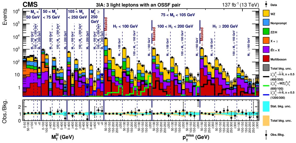
Figure 8. Observed and expected yields across the search regions in events with three light leptons, at least two of which form an OSSF pair (3 \ell A). Several signal models are shown superimposed. They correspond to \tilde{\chi}_1^\pm \tilde{\chi}_2^0 production with slepton-mediated decays in the flavor-democratic hypothesis for a compressed \delta m = 50 GeV (black line) and uncompressed \delta m = 900 GeV (blue line) scenario, and for WZ-mediated decays in an uncompressed \delta m = 500 GeV scenario (green line). Bins labeled as “Masked” are not considered in the interpretation of the results because of overlap with the WZ control region. The legends specify the masses of \tilde{\chi}_2^0 and \tilde{\chi}_1^0 for the shown signal distributions as (m_{\tilde{\chi}_2^0}/m_{\tilde{\chi}_1^0}) .
