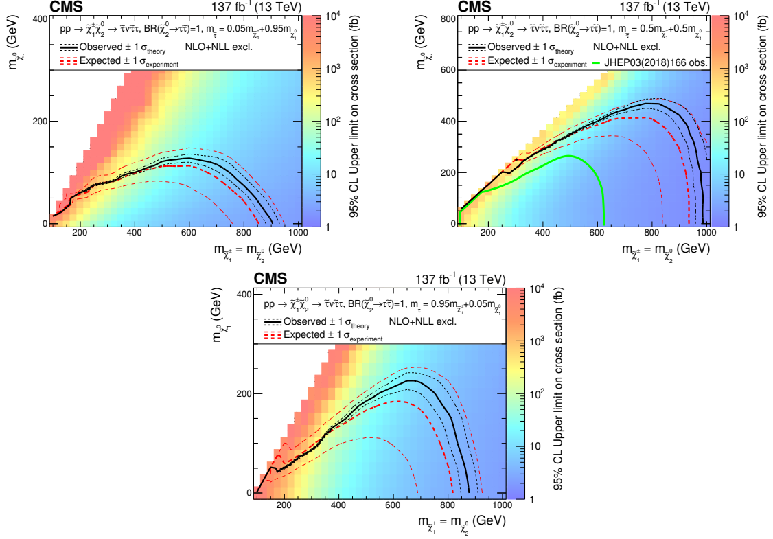
Figure 18. Interpretation of the results for \tilde{\chi}_1^{\pm 0} \tilde{\chi}_2^0 production with \tau -dominated slepton-mediated decays, and the parameter governing the mass splittings being x = 0.05 (upper left), x = 0.5 (upper right) and x = 0.95 (lower). The shading in the m_{\tilde{\chi}_1^{\pm 0}} versus m_{\tilde{\chi}_2^0} plane indicates the 95% CL upper limits on the \tilde{\chi}_1^{\pm 0} \tilde{\chi}_2^0 production cross sections. The contours delineate the mass regions excluded at 95% CL when assuming cross sections computed at NLO plus NLL. The observed, observed \pm 1\sigma_{\text{theory}} ( \pm 1 standard deviation of the theoretical cross sections), median expected, and expected \pm 1\sigma_{\text{experiment}} bounds are shown in black and red. The median expected bound obtained with the search region strategy is shown in blue. The observed limits obtained in the CMS analysis using 2016 data [20] are shown in green, which only included interpretations in the x = 0.5 case.
