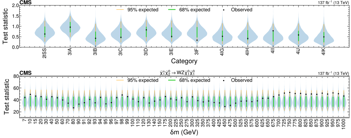
Figure 15. Expected test statistic distribution for a background-only fit compared to the observed test statistic value, drawn as black dots, for the search regions in each event category (upper plot) and the neural network targeting WZ-mediated superpartner decays for each \delta m evaluation (lower plot). The gray shaded area represents the (symmetrized) probability density of the expected test statistic distribution, with 68 and 95% expected ranges respectively drawn in green and orange.
