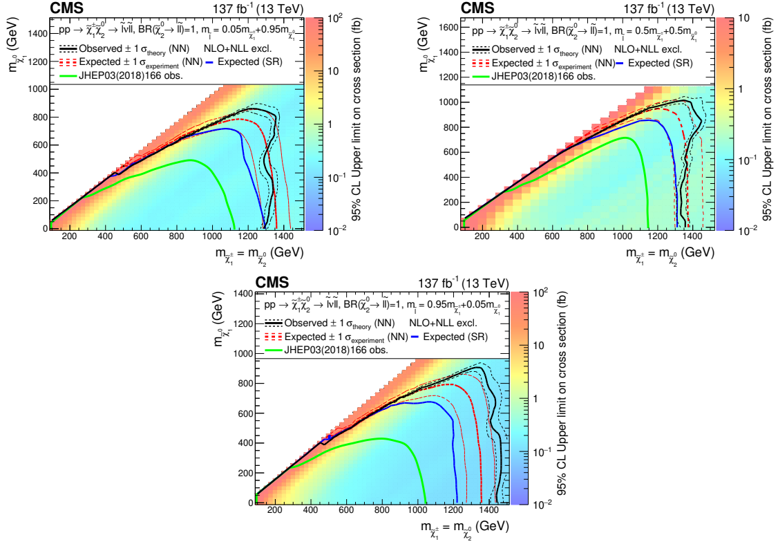
Figure 16. Interpretation of the results for \tilde{\chi}_1^{\pm}\tilde{\chi}_2^0 production with flavor-democratic slepton-mediated decays, and the parameter governing the mass splittings being x = 0.05 (upper left), x = 0.5 (upper right) and x = 0.95 (lower). The shading in the m_{\tilde{\chi}_1^{\pm}} versus m_{\tilde{\chi}_2^0} plane indicates the 95% CL upper limit on the \tilde{\chi}_1^{\pm}\tilde{\chi}_2^0 production cross sections. The contours delineate the mass regions excluded at 95% CL when assuming cross section computed at NLO plus NLL. All masses below the contours are excluded. The observed, observed \pm 1\sigma_{\text{theory}} ( \pm 1 standard deviation of the theoretical cross sections), median expected, and expected \pm 1\sigma_{\text{experiment}} bounds obtained with the neural network strategy are shown in black and red. The median expected bound obtained with the search region strategy is shown in blue. The observed limits obtained in the CMS analysis using 2016 data [20] are shown in green.
