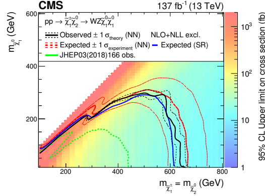
Figure 19. Interpretation of the results for \tilde{\chi}_1^{\pm}\tilde{\chi}_2^0 production with WZ-mediated decays. The shading in the m_{\tilde{\chi}_1^0} versus m_{\tilde{\chi}_2^0} plane indicates the 95% CL upper limits on the \tilde{\chi}_1^{\pm}\tilde{\chi}_2^0 production cross sections. The contours delineate the mass regions excluded at 95% CL when assuming cross sections computed at NLO plus NLL. The observed, observed \pm 1\sigma_{\text{theory}} ( \pm 1 standard deviation of the theoretical cross sections), median expected, and expected \pm 1\sigma_{\text{experiment}} bounds obtained with the neural network strategy are shown in black and red. The median expected bound obtained with the search region strategy is shown in blue. The observed limits obtained in the CMS analysis using 2016 data [20] are shown in green.
