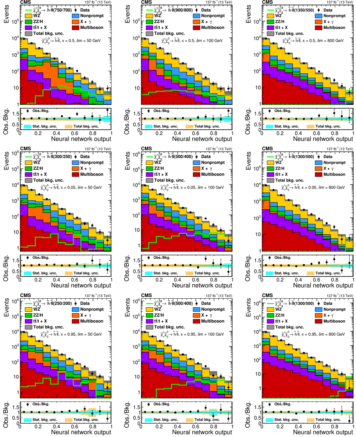
Figure 6. Observed and expected yields as functions of the output of the neural network used to search for \tilde{\chi}_1^{\pm 0} \tilde{\chi}_2^0 production with slepton-mediated decays at x = 0.5 (upper), 0.05 (middle), and 0.95 (lower), evaluated at \delta m = 50 GeV (left), 100 GeV (center), and 800 GeV (right). The legends specify the masses of \tilde{\chi}_2^0 and \tilde{\chi}_1^0 for the shown signal distributions as (m_{\tilde{\chi}_2^0}/m_{\tilde{\chi}_1^0}) .
