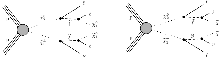
Figure 1. Production of \tilde{\chi}_1^\pm \tilde{\chi}_2^0 with subsequent decays via sleptons (left) and a slepton and a sneutrino (right).
