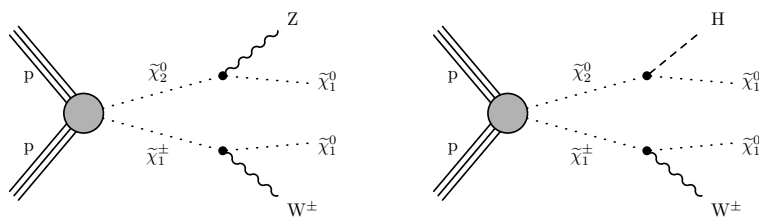
Figure 2. Production of \tilde{\chi}_1^\pm \tilde{\chi}_2^0 with subsequent decay of \tilde{\chi}_1^\pm via a W boson and \tilde{\chi}_2^0 via a Z boson (left) or H boson (right).
