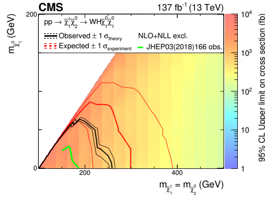
Figure 20. Interpretation of the results for \tilde{\chi}_1^{\pm}\tilde{\chi}_2^0 production with WH-mediated decays. The shading in the m_{\tilde{\chi}_1^0} versus m_{\tilde{\chi}_2^0} plane indicates the 95% CL upper limits on the \tilde{\chi}_1^{\pm}\tilde{\chi}_2^0 production cross sections. The contours delineate the mass regions excluded at 95% CL when assuming cross sections computed at NLO plus NLL. The observed, observed \pm 1\sigma_{\text{theory}} ( \pm 1 standard deviation of the theoretical cross sections), median expected, and expected \pm 1\sigma_{\text{experiment}} bounds are shown in black and red. The observed limits obtained in the CMS analysis using 2016 data [20] are shown in green.
