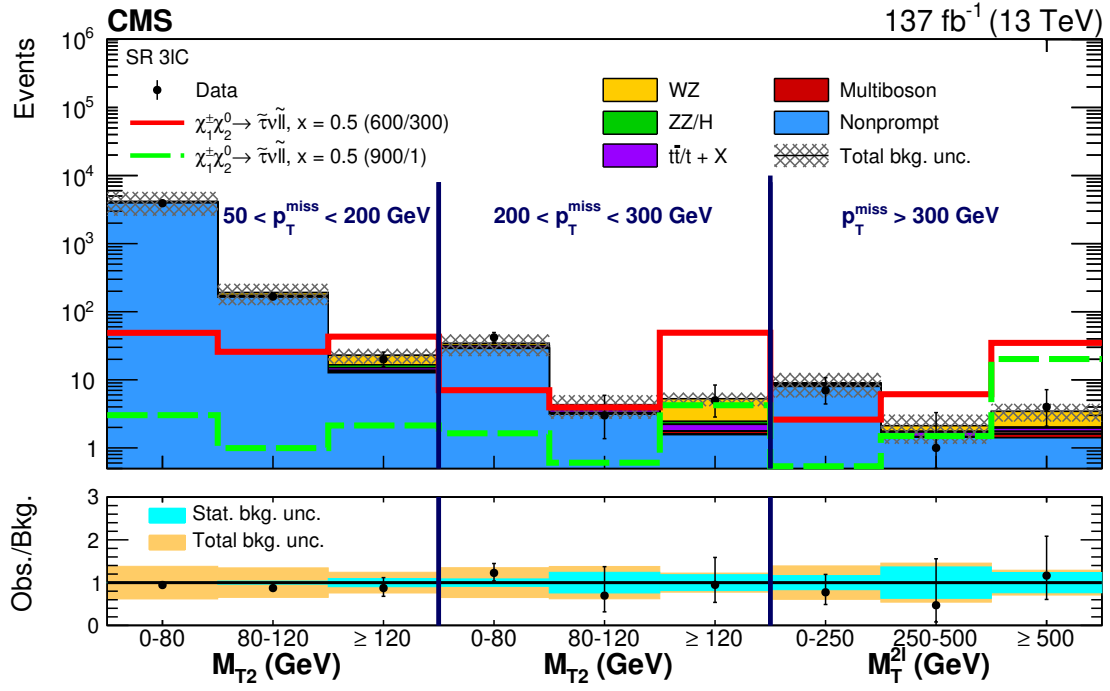
Figure 10. Observed and expected yields across the search regions in events with a \mu^+\mu^- or e^+e^- pair and an additional \tau_h candidate ( 3\ell C ). Several signal models are shown superimposed. They correspond to \tilde{\chi}_1^\pm\tilde{\chi}_2^0 production with slepton-mediated decays in the \tau lepton enriched hypothesis for a compressed \delta m = 300 GeV (red line) and uncompressed \delta m = 900 GeV (green dashed line) scenario. The legends specify the masses of \tilde{\chi}_2^0 and \tilde{\chi}_1^0 for the shown signal distributions as (m_{\tilde{\chi}_2^0}/m_{\tilde{\chi}_1^0}) .
