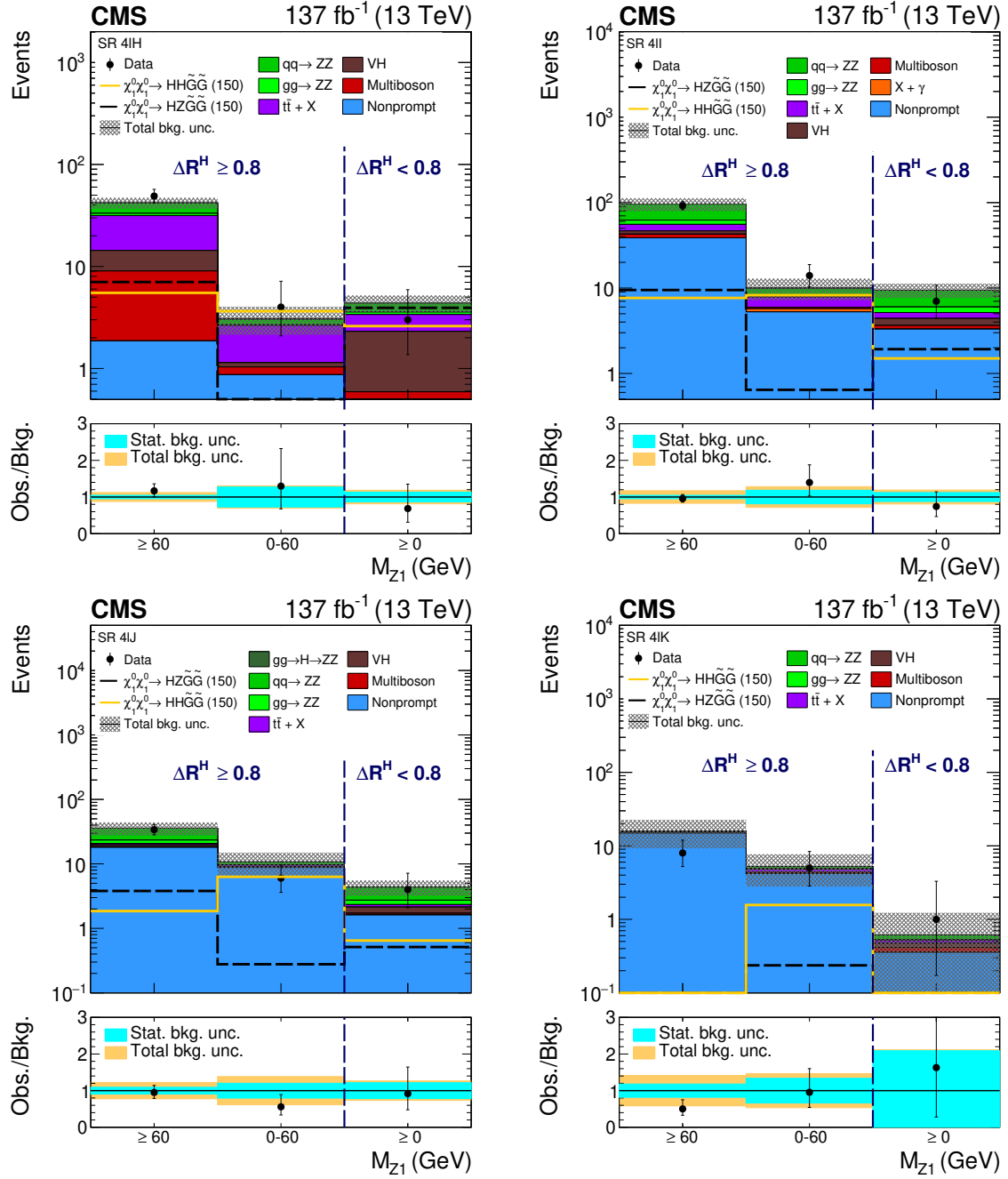
Figure 14. Observed and expected yields across the search regions in events with four light leptons not forming two OSSF pairs (4ℓH, upper left), events with three light leptons and a \tau_h candidate (4ℓI, upper right), forming two OSSF pairs (4ℓJ, lower left), and forming one or less OSSF pairs (4ℓK, lower right). Several signal models are shown superimposed. They correspond to Higgsino pair production with decays to HZ (dashed black line, Higgsino mass of 150 GeV), and HH (dark yellow line, Higgsino mass of 150 GeV).
