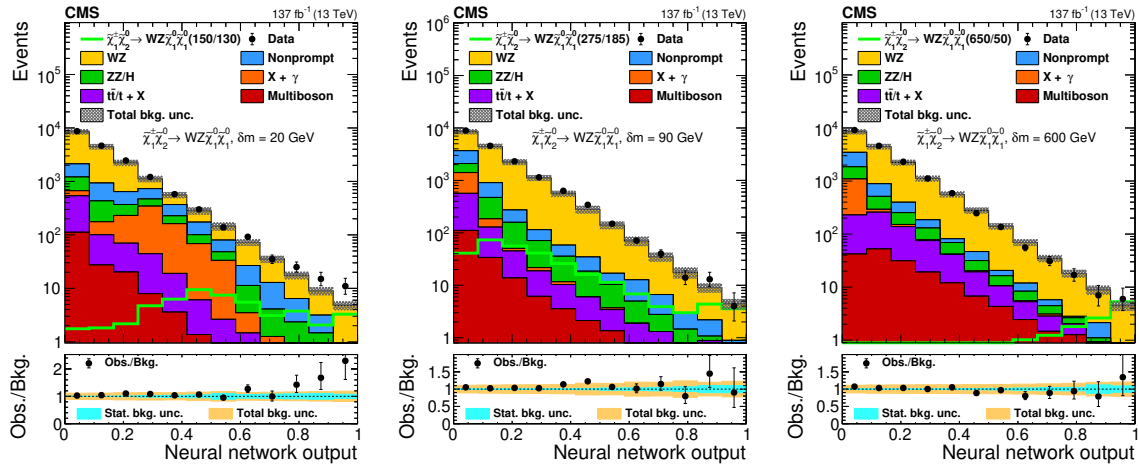
Figure 5. Observed and expected yields as functions of the output of the neural network used to search for \tilde{\chi}_1^{\pm 0} \tilde{\chi}_2^0 production with WZ-mediated decays, evaluated at \delta m = 20 GeV (left), 90 GeV (center), and 600 GeV (right). The legends specify the masses of \tilde{\chi}_2^0 and \tilde{\chi}_1^0 for the shown signal distributions as (m_{\tilde{\chi}_2^0}/m_{\tilde{\chi}_1^0}) . The top panels show only the total uncertainty in the background prediction, while the lower panels show the total and statistical uncertainties separately. The following abbreviations are used in the legends of this and the following figures: “bkg.” stands for background, “unc.” for uncertainty and “obs.” for observed.
