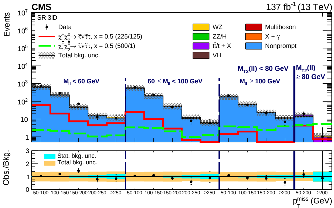
Figure 11: Observed and expected yields across the search regions in events with an e^\pm \mu^\mp pair and a \tau_h candidate (3ℓD). Several signal models are shown superimposed. They correspond to \tilde{\chi}_1^\pm \tilde{\chi}_2^0 production with slepton-mediated decays in the \tau lepton dominated hypothesis for a compressed \delta m = 100 GeV (red line) and uncompressed \delta m = 500 GeV (green dashed line) scenario. The legends specify the masses of \tilde{\chi}_2^0 and \tilde{\chi}_1^0 for the shown signal distributions as (m_{\tilde{\chi}_2^0}/m_{\tilde{\chi}_1^0}) .
