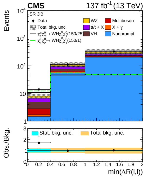
Figure 9: Observed and expected yields across the search regions in events with three light leptons, none of which form an OSSF pair (3ℓB). Several signal models are shown superimposed. They correspond to \tilde{\chi}_1^\pm \tilde{\chi}_2^0 production with WH-mediated decays for scenarios corresponding to a H boson like mass splitting \delta m = 125 \text{ GeV} (black line) and a slightly less compressed \delta m = 150 \text{ GeV} (green dashed line) scenario. The legends specify the masses of \tilde{\chi}_2^0 and \tilde{\chi}_1^0 for the shown signal distributions as (m_{\tilde{\chi}_2^0}/m_{\tilde{\chi}_1^0}) .
