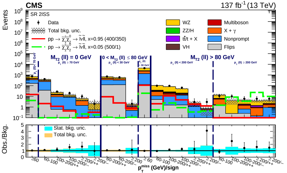
Figure 7: Observed and expected yields across the search regions in events with two same-sign light leptons (2ℓSS). Several signal models are shown superimposed. They correspond to \tilde{\chi}_1^\pm \tilde{\chi}_2^0 production with slepton-mediated decays in the flavor-democratic hypothesis for a compressed \delta m = 50 GeV (red line) and uncompressed \delta m = 500 GeV (green dashed line) scenario. The legends specify the masses of \tilde{\chi}_2^0 and \tilde{\chi}_1^0 for the shown signal distributions as (m_{\tilde{\chi}_2^0}/m_{\tilde{\chi}_1^0}) .
