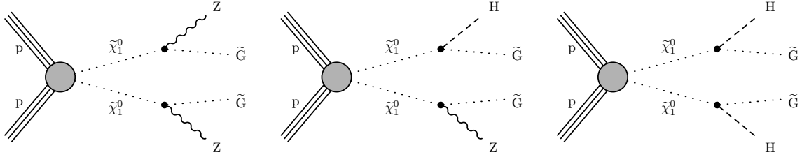
Figure 3: Effective \tilde{\chi}_1^0 pair production with decays mediated by Z or H bosons.
