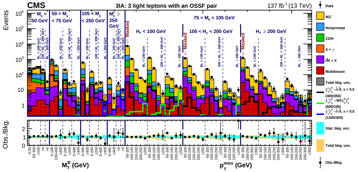
Figure 8: Observed and expected yields across the search regions in events with three light leptons, at least two of which form an OSSF pair (3ℓA). Several signal models are shown superimposed. They correspond to \tilde{\chi}_1^\pm \tilde{\chi}_2^0 production with slepton-mediated decays in the flavor-democratic hypothesis for a compressed \delta m = 50 GeV (black line) and uncompressed \delta m = 900 GeV (blue line) scenario, and for WZ-mediated decays in an uncompressed \delta m = 500 GeV scenario (green line). Bins labeled as “Masked” are not considered in the interpretation of the results because of overlap with the WZ control region. The legends specify the masses of \tilde{\chi}_2^0 and \tilde{\chi}_1^0 for the shown signal distributions as (m_{\tilde{\chi}_2^0}/m_{\tilde{\chi}_1^0}) .
