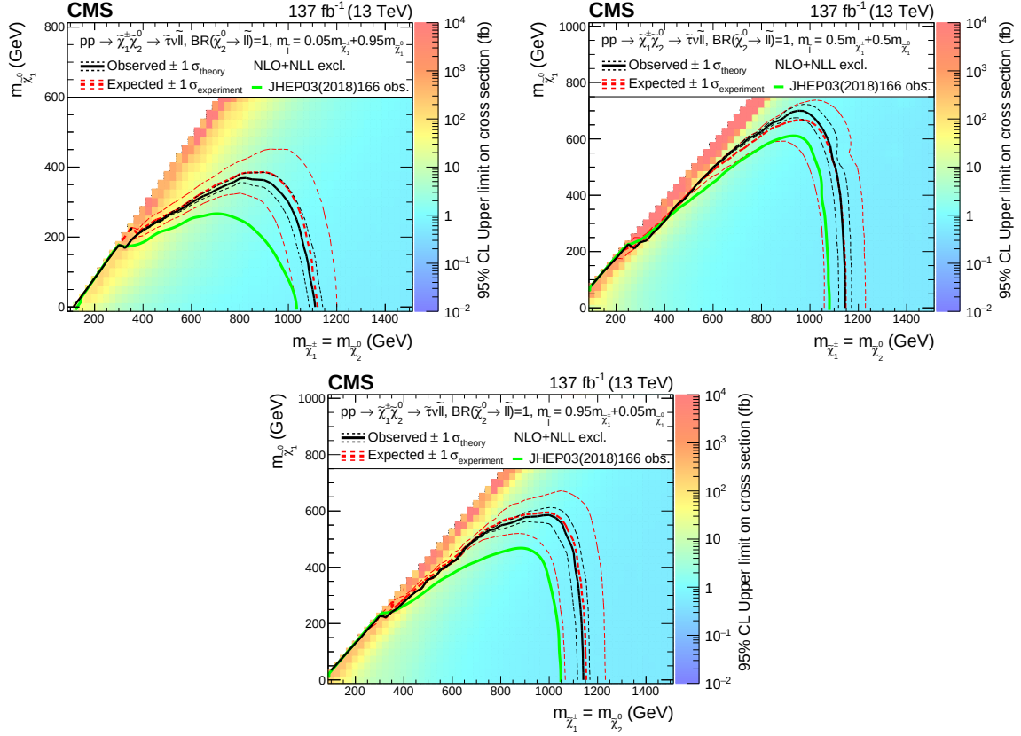
Figure 17: Interpretation of the results for \tilde{\chi}_1^\pm \tilde{\chi}_2^0 production with \tau -enriched slepton-mediated decays, and the parameter governing the mass splittings being x = 0.05 (upper left), x = 0.5 (upper right) and x = 0.95 (lower). The shading in the m_{\tilde{\chi}_1^\pm} versus m_{\tilde{\chi}_2^0} plane indicates the 95% CL upper limits on the \tilde{\chi}_1^\pm \tilde{\chi}_2^0 production cross sections. The contours delineate the mass regions excluded at 95% CL when assuming cross sections computed at NLO plus NLL. The observed, observed \pm 1\sigma_{\text{theory}} ( \pm 1 standard deviation of the theoretical cross sections), median expected, and expected \pm 1\sigma_{\text{experiment}} bounds are shown in black and red. The observed limits obtained in the CMS analysis using 2016 data [20] are shown in green.
