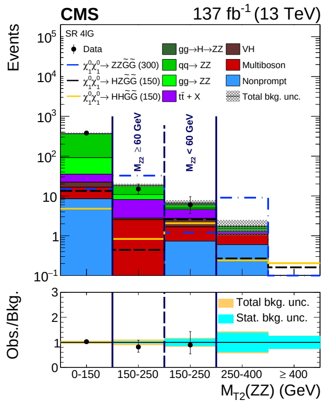
Figure 13: Observed and expected yields across the search regions in events with four light leptons, including 2 separate OSSF pairs (4ℓG). Several signal models are shown superimposed. They correspond to Higgsino pair production with decays to ZZ (blue dotted line, Higgsino mass of 300 GeV), HZ (black dashed line, Higgsino mass of 150 GeV), and HH (dark yellow line, Higgsino mass of 150 GeV).
