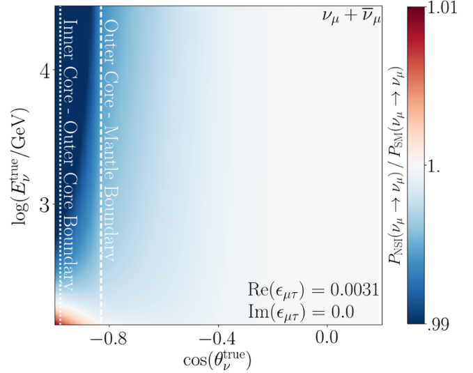
FIG. 1. Muon neutrino oscillogram—an example of how NSI modify predicted neutrino fluxes. Shown here is the probability ratio of NSI-modified oscillations to the SM prediction for atmospheric neutrinos [chosen value is \text{Re}(\epsilon_{\mu\tau}) = 0.0031 , \text{Im}(\epsilon_{\mu\tau}) = 0.0 , the 90% CL bound on positive \text{Re}(\epsilon_{\mu\tau}) ]. Effects include flux disappearance at energies of 1 TeV and above for events crossing the largest Earth baselines [ \cos(\theta) = -1 ] and flux enhancement at \sim 100 GeV. Note that the neutrino true energy range corresponds to the stated muon proxy energy range, and that the maximum disappearance for this value of \epsilon_{\mu\tau} is \sim 3.4\% .
