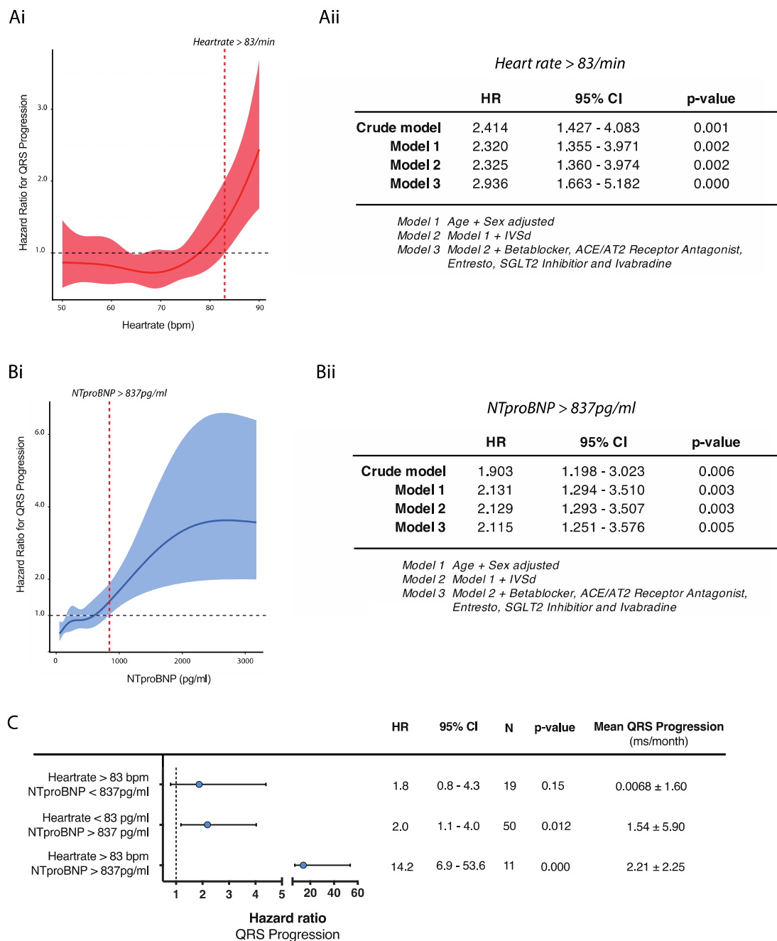
Fig. 2 Ai Prediction function by restricted cubic splines for the continuous relationship between QRS width progression and heart rate. Restricted cubic splines were used to define cut-offs for patients at risk. Datasets were stratified according to the presence or absence of QRS width progression. Aii Cox proportional hazard model for patients with a heart rate > 83/min and QRS width progression step-
