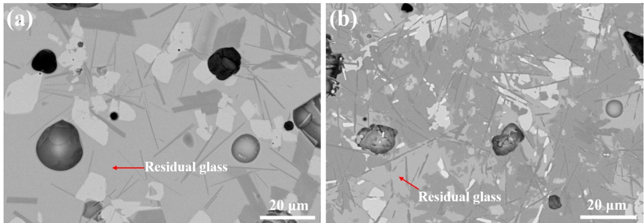
Fig. 4-3. SEM micrographs of dilatometer samples, (a) glass H sintered at 850 °C for 10 h, (b) the annealed glass H sample sintered at 850 °C for 10 h then aged at 800 °C for 1000 h.
