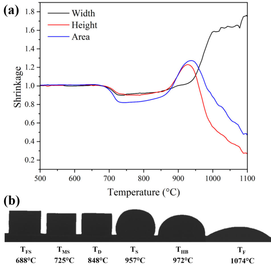
Fig. 4-49. HSM analysis (TOMMIplus) for HS2S20 glass composite sealant on Crofer 22 APU substrate recorded at 5 °C/min, (a) shrinkage curves, (b) Shadow images of the sample at the fixed temperature
