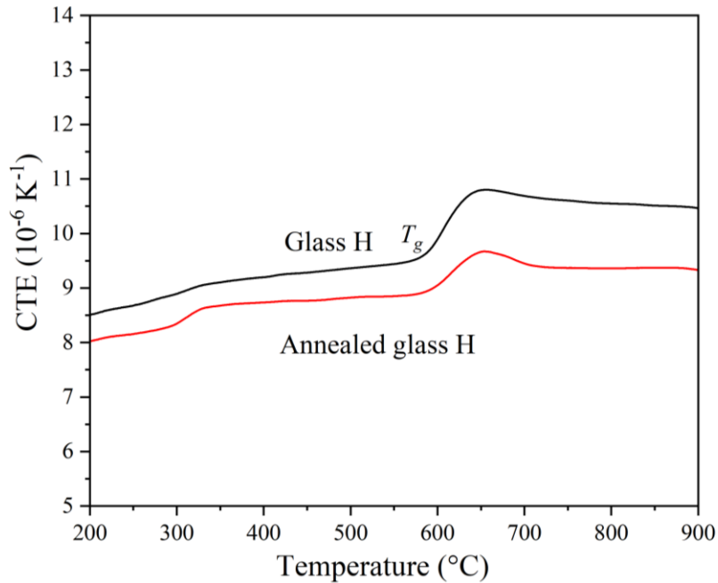
Fig. 4-2. Dilatometer plots of the sintered glass H rod (850 °C, 10 h) and glass H aged sample (850 °C, 10 h + 800 °C, 1000 h)
