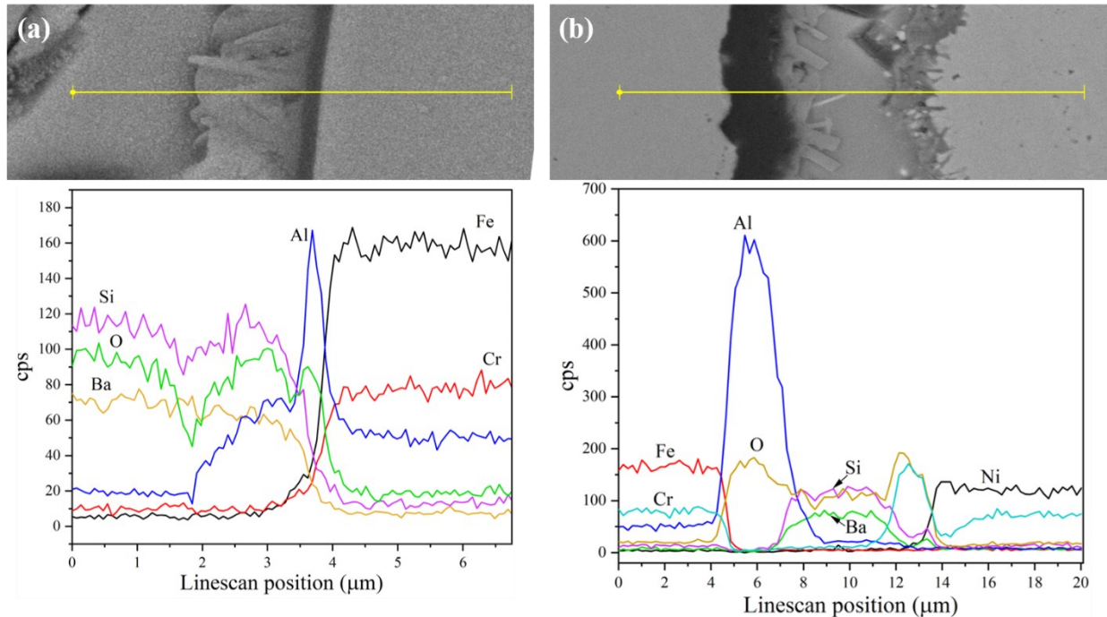
Fig. 4-18. Line scans through the interface between HNC30 and Aluchrom (a), HNC30 and pre-Aluchrom (b)
