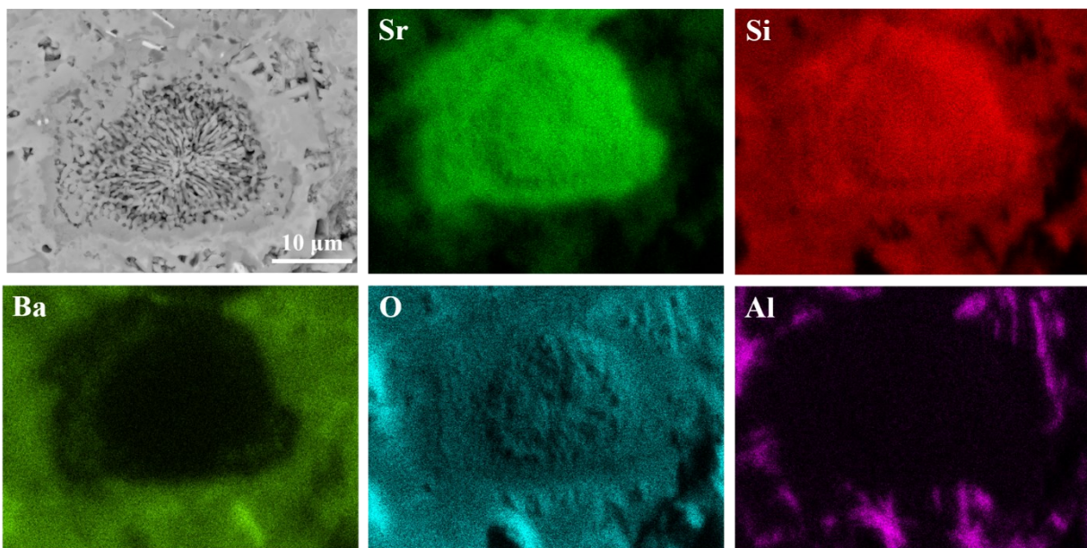
Fig. 4-48. SEM-EDS maps of the HS2S20A sample
