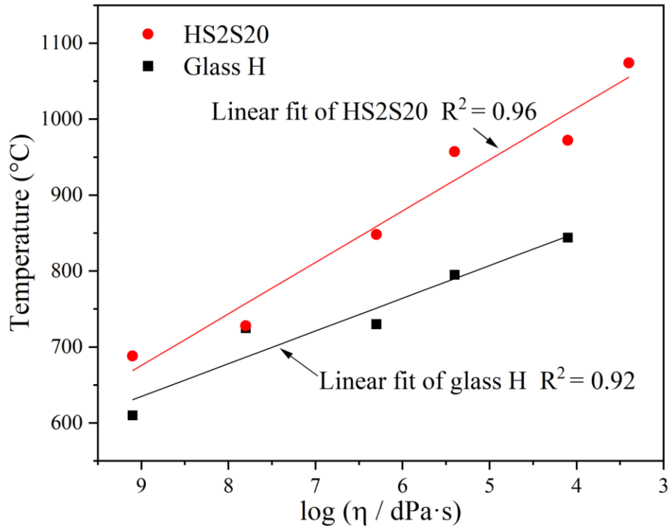
Fig. 4-50. Viscosity-temperature curves of glass H and composite sealant HS2S20
