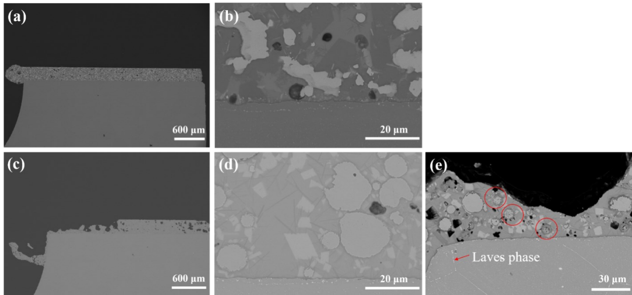
Fig. 4-20. SEM images of cross sections of HA940 (a, b) and HNC30 (c-e) samples after torsion tests, overview on the left and magnification on the right
