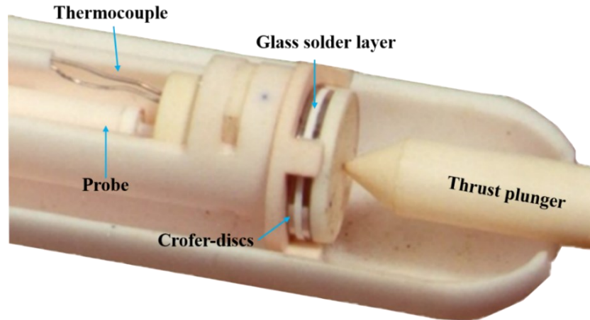
Fig. 3-2. Probe head of the sinking dilatometer
