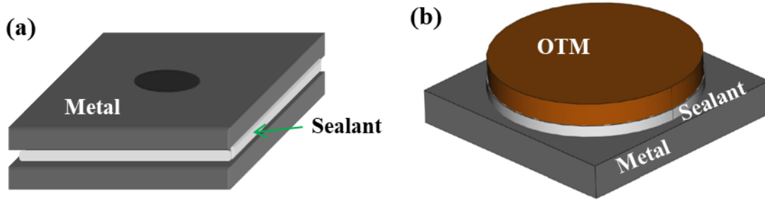
Fig. 3-5. Schematic illustrations of joining geometries: (a) sealant sealing metal plates for gas-tightness testing, (b) sealant assembled with OTM and metallic support
