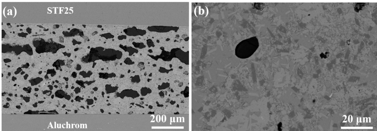
Fig. 4-44. Joint STF25/HBS30/Aluchrom joined at 920 °C for 15 min
