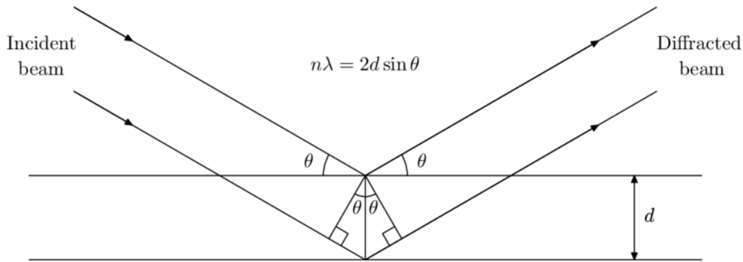
Fig. 3-1. Schematic illustration of Bragg's Law [114]
