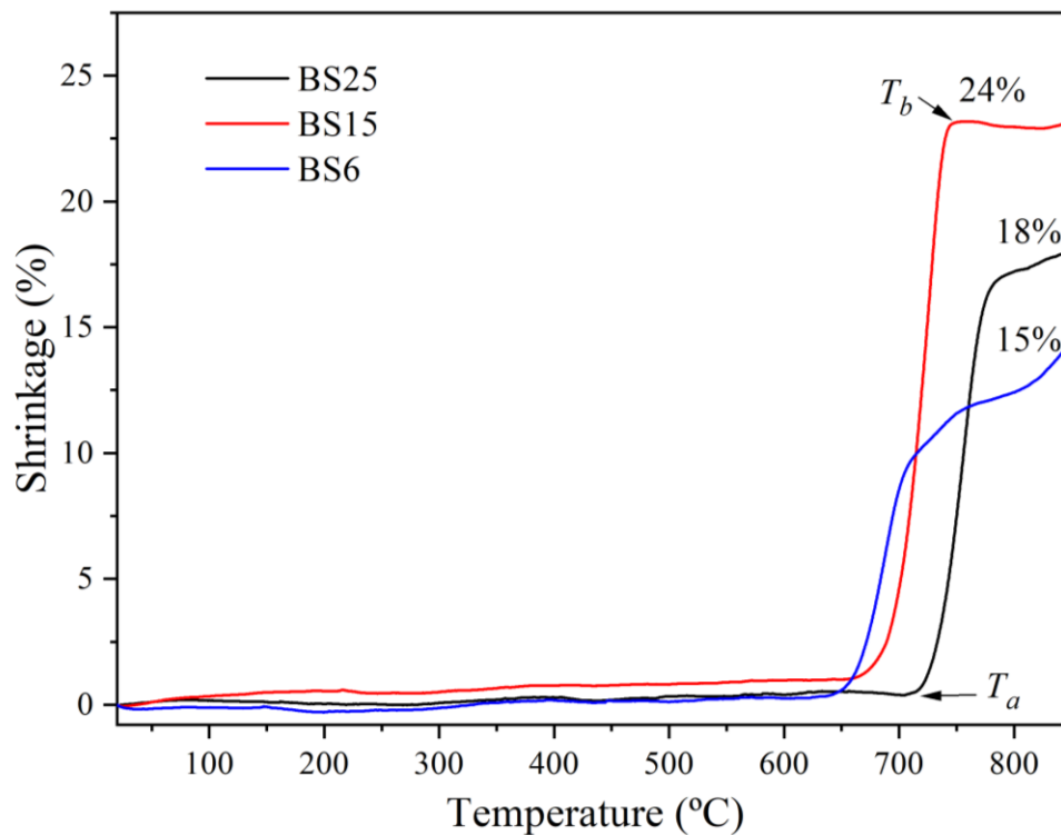
Fig. 4-60. Sinking dilatometry plots of BS glasses
