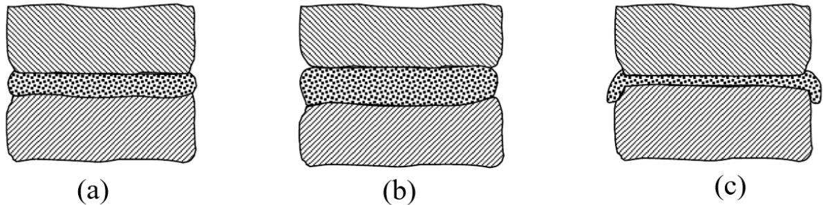
Fig. 2-8. Schematic illustrations of cross sections of joining geometry: (a) ideal joint, (b) too high viscosity (thick joining layer), (c) too low joining viscosity (thin joining layer and bead drop) [67]
