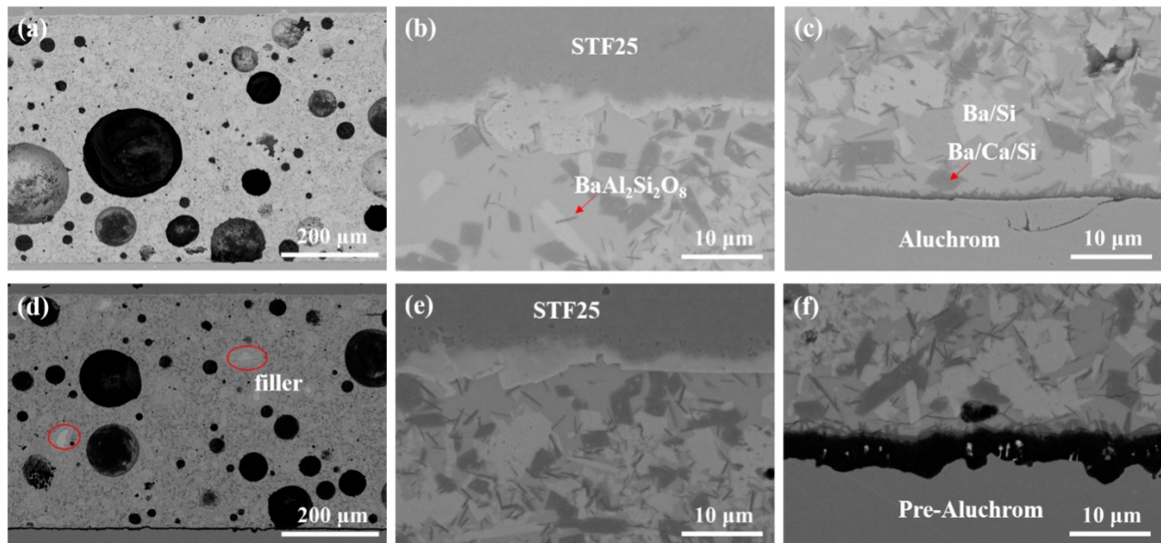
Fig. 4-39. Joints STF25/HBS30/Aluchrom (a-c) and STF25/HBS30/pre-oxidized Aluchrom (d-f); both joints jointed at 960 °C for 5 min.
