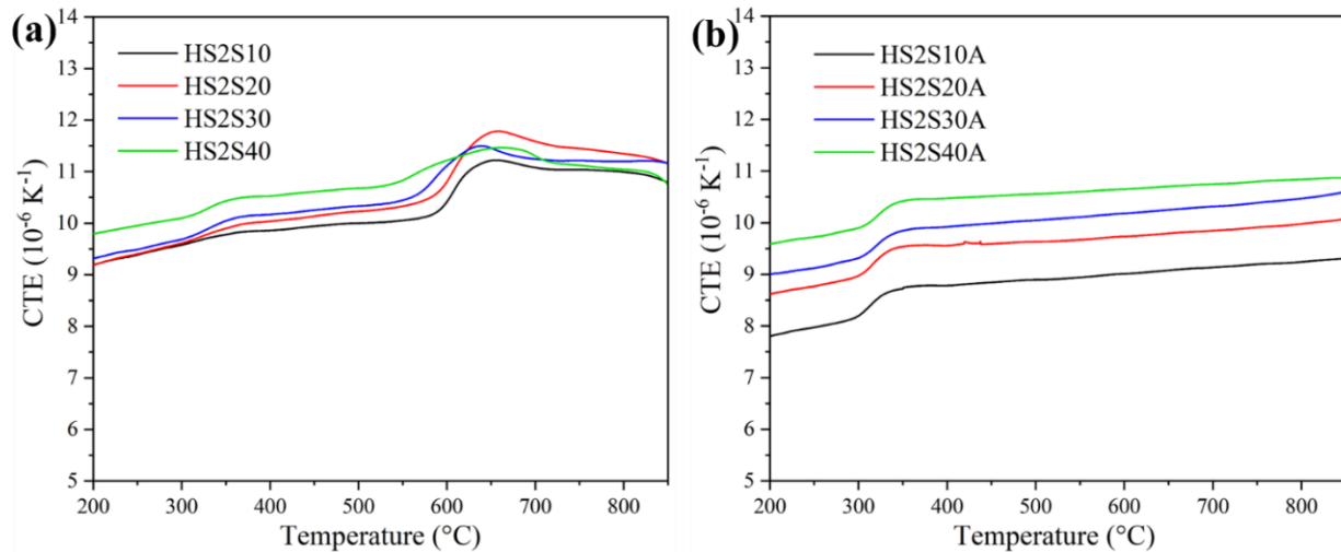
Fig. 4-46. CTE curves for composites samples sintered (a) and annealed (b)
