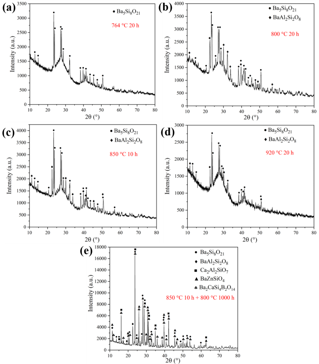
Fig. 4-4. Glass H after different heat-treatments for crystallization analysis, (a) XRD pattern of glass H after heating at 764 °C for 20 hours, (b) XRD pattern of glass H after heating at 800 °C for 20 hours, (c) XRD pattern of glass H after heating at 850 °C for 10 hours, (d) XRD pattern of glass H after heating at 920 °C for 20 hours, (e) XRD pattern of glass H after heat-treatment at 850 °C for 10 hours followed by 800 °C for 1000 hours, with same heating and cooling rate of 2 °C/min.
