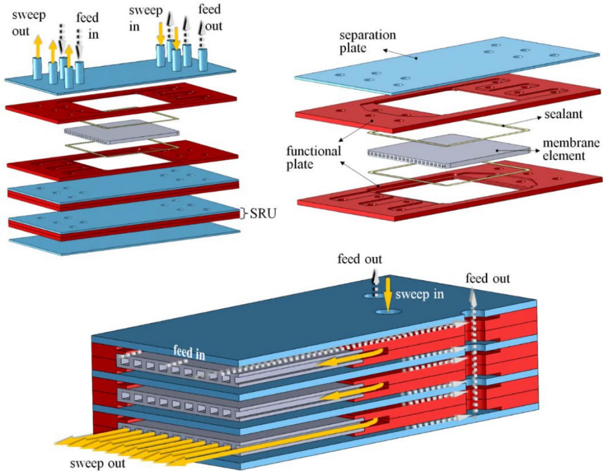
Fig. 2-3. Design concept for the operation of a planar membrane module stack in 4-end mode (top left), single reproduction unit (SRU, top right), and quarter section with illustrated flow of feed and sweep gas [11].
