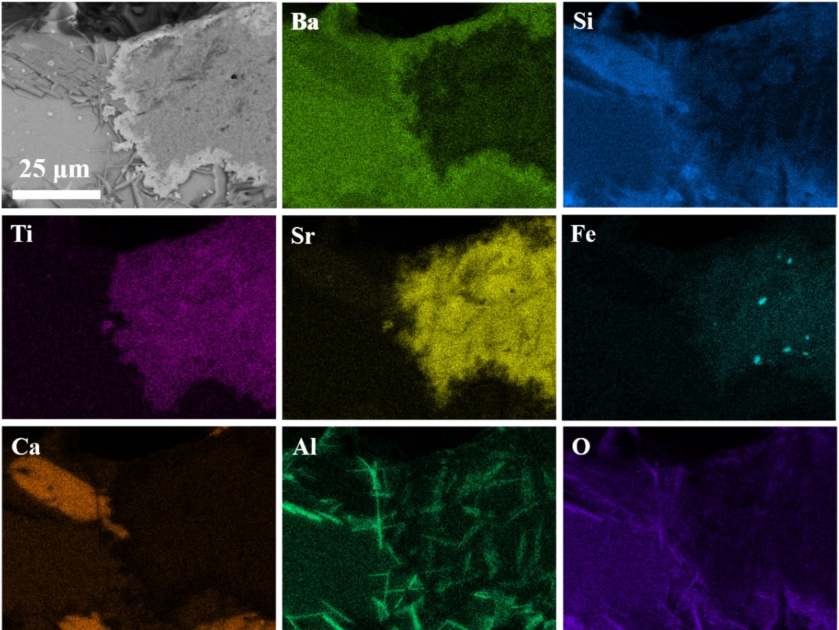
Fig. 4-11. SEM-EDS maps of the H10STF25
