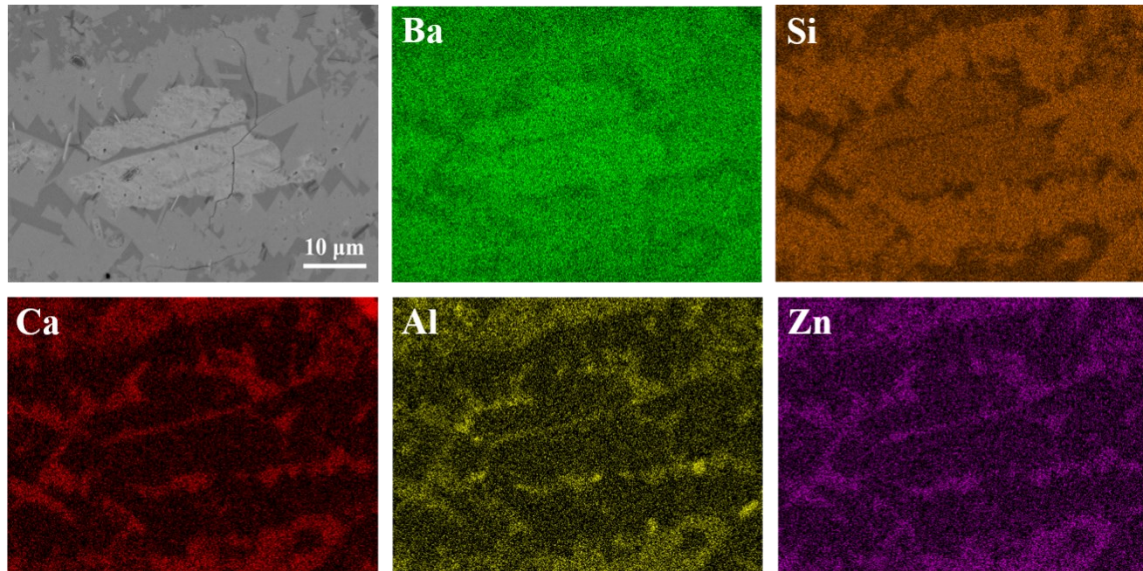
Fig. 4-40. SEM-EDS maps of the sealant HBS30 from STF25/HBS30/pre-Aluchrom joint (960 °C, 5 min) for analyzing filler BaSiO 3
