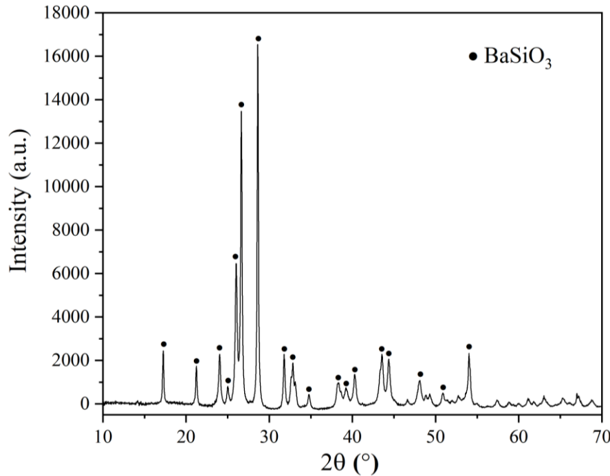
Fig. 4-33. XRD pattern of the BaSiO 3 filler
