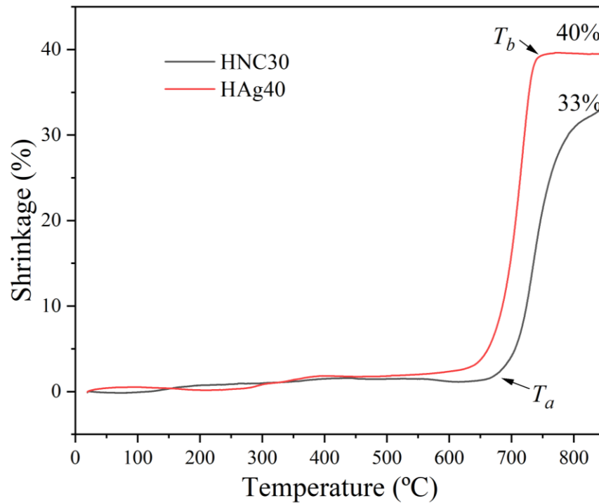
Fig. 4-14. Sinking dilatometer of HAg40 and HNC30
