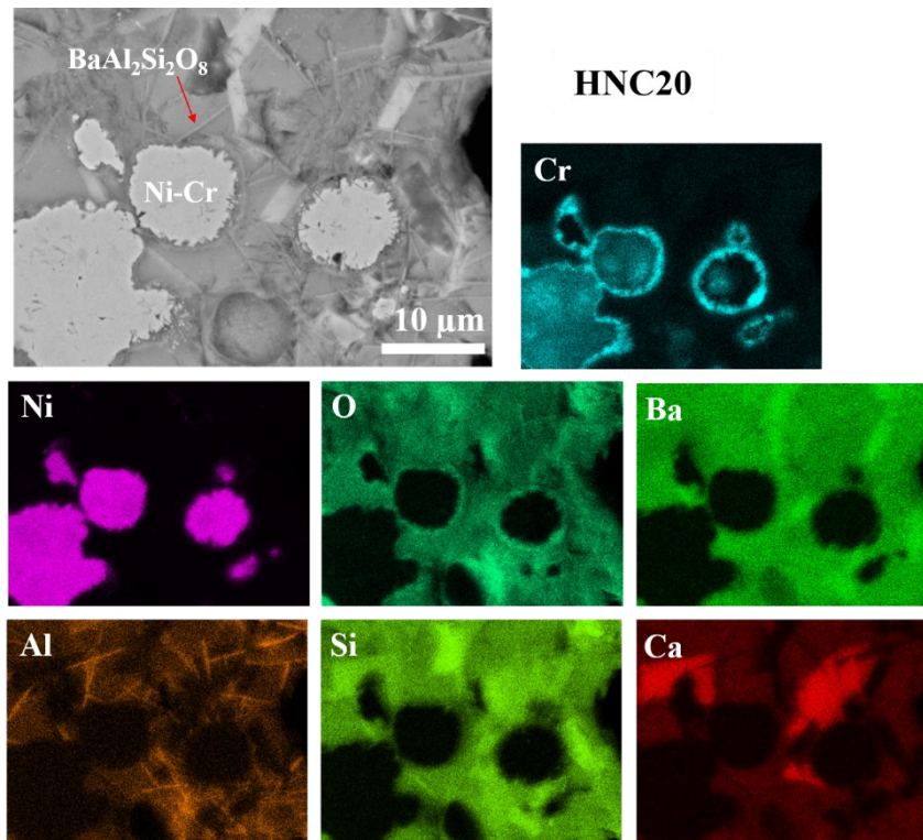
Fig. 4-9. SEM-EDS maps of the HNC20 sample
