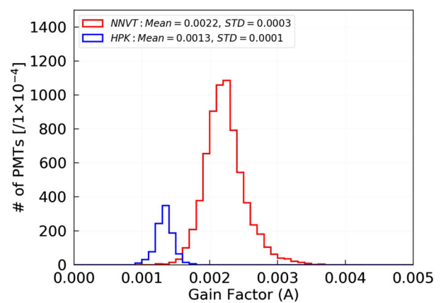
(b) Gain factor A for the gain of the qualified PMTs. Red: NNVT; blue: HPK.
