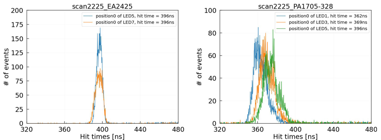
Fig. 40 PMT hit time (relative TT) distribution of a single NNV and HPK PMT directly measured in the scanning station with different LEDs (locations) at azimuthal angle \phi = 0 . Left: HPK (blue: 5th LED; orange: 7th LED); right: NNV (blue: 1st LED; orange: 3rd LED; green: 5th LED)
