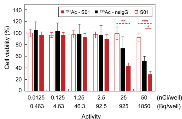
Fig. 4 Cell viability after 4-day incubation times with 225 Ac-S01, 225 Ac-nsIgG, and S01. (*), (**) and (***) indicate groups that are significantly different with p < 0.05 , p < 0.005 and p < 0.001 , respectively (one-tailed Welch's t -test). The experiments were performed in triplicates, error bars represent one standard deviation of the measurements.
