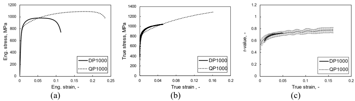
Figure 4. The tensile properties from uniaxial tensile tests, (a) engineering stress-strain curves, (b) true stress-strain curves, and (c) r-value curves of QP1000 in comparison with DP1000.
