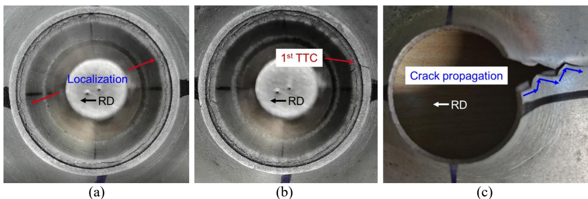
Figure 6. Edge fracture pattern and locations on smooth edges for DP1000 (a) after strong localization, (b) the moment when the first through-thickness crack occurs, and (c) crack propagation with blue marks.
