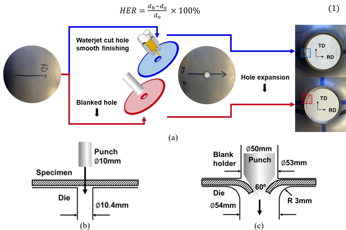
Figure 3. Schematic diagram of (a) the edge fracture characterization approach, (b) cross-section view of the hole blanking, and (c) cross-section view of the hole expansion process.
