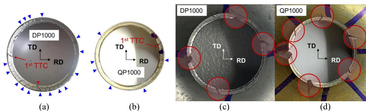
Figure 8. Edge fracture pattern and locations on blanked edges for (a) DP1000 and (b) QP1000 with blue marks for minor cracks, (c) further expanded with four major cracks at the punched edge of DP1000, and (d) QP1000.
