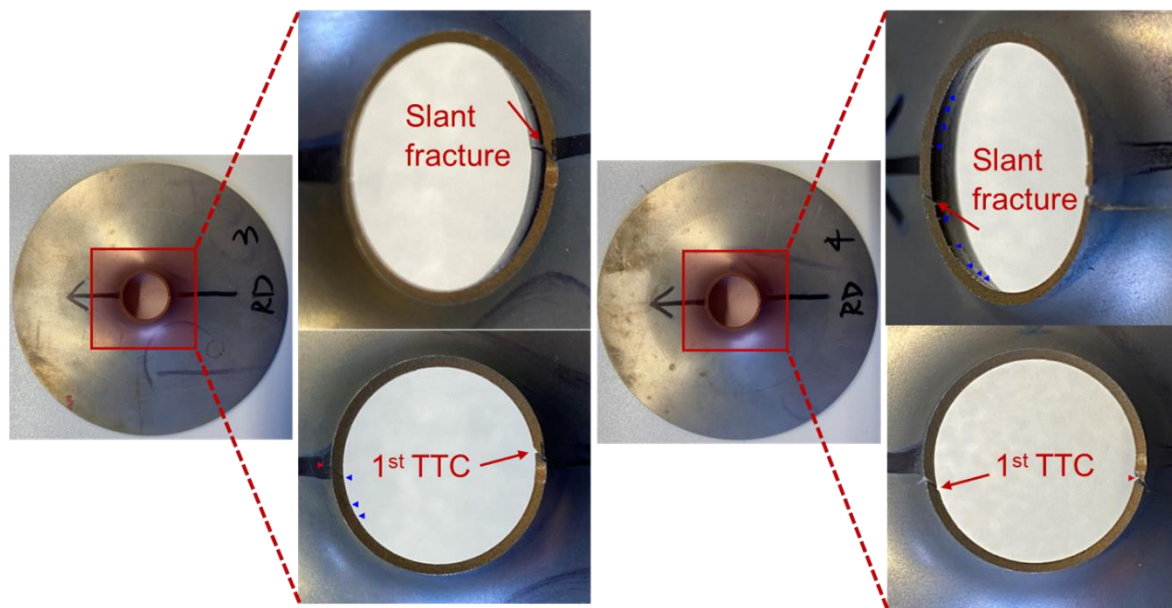
Figure 7. Edge fracture pattern and locations on smooth edges for QP1000 after first through-thickness crack, and blue marks for minor cracks.
