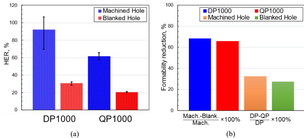
Figure 5. HER values analysis (a) of the punched and machined holes for DP1000 and QP1000, (b) the formability reduction from smooth edge to punched edge for each material, and from DP1000 to QP1000 for each edge condition.
