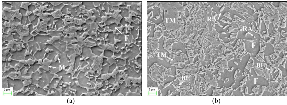
Figure 1. Microstructure of (a) DP1000 [24] with martensite (M) and ferrite (F) phases indicated, and (b) QP1000 with retained austenite (RA), tempered martensite (TM), bainitic ferrite (BF) phases indicated.
