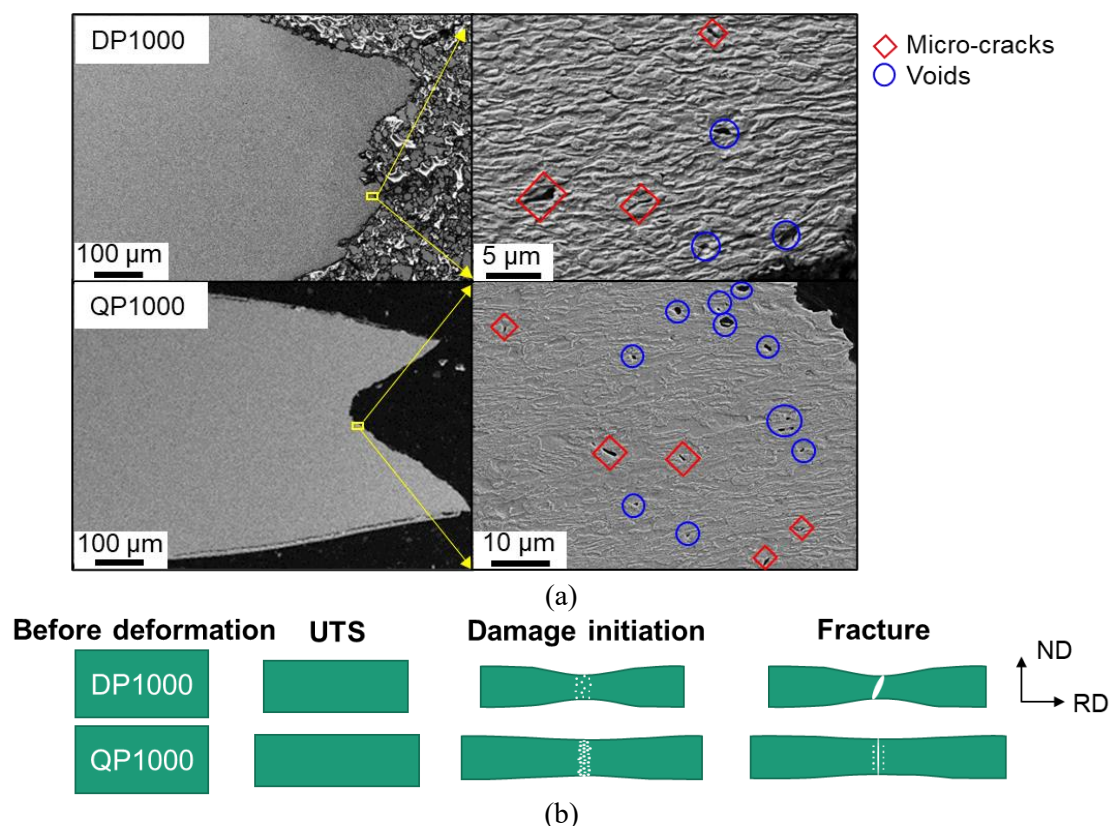
Figure 9. Microstructure-level damage mechanism analysis: (a) SEM fractography of fractured specimens with the red and blue indicators pointing out the micro-cracks and voids, respectively, and (b) schematic drawing of the relationship pattern during uniaxial tension for DP1000 and QP1000.
