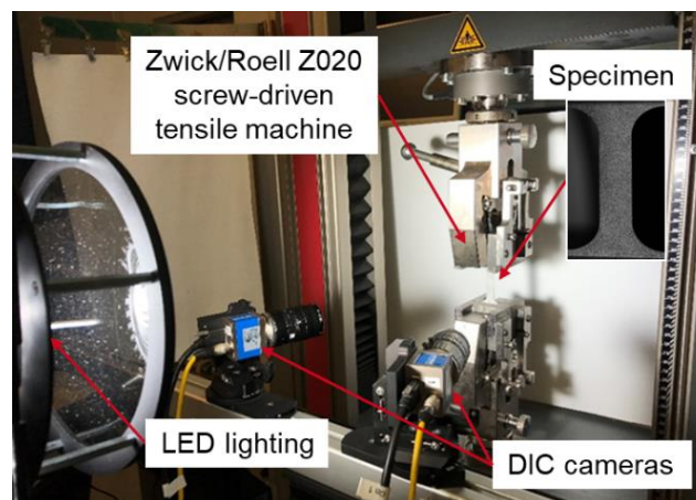
Figure 2. Uniaxial tensile testing set-up with stereo-DIC system and lighting.
