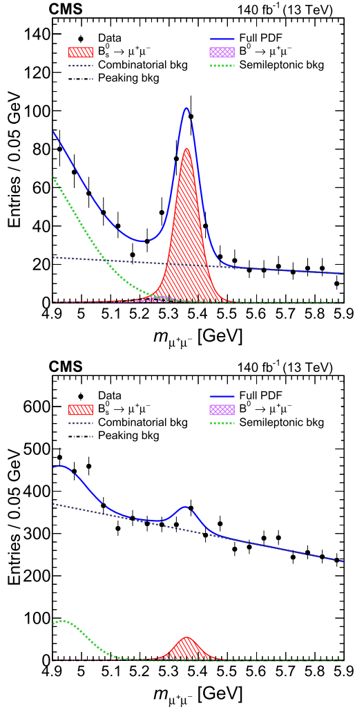
Fig. 3. The projections on the dimuon mass axis of the fit to the branching fraction for the d_{\text{MVA}} > 0.99 (upper) and 0.99 > d_{\text{MVA}} > 0.90 (lower) categories. The solid blue curves represent the corresponding projections of the final fit model, while the individual components of the fit are represented by the dashed curves (backgrounds) and hatched histograms (signals).
