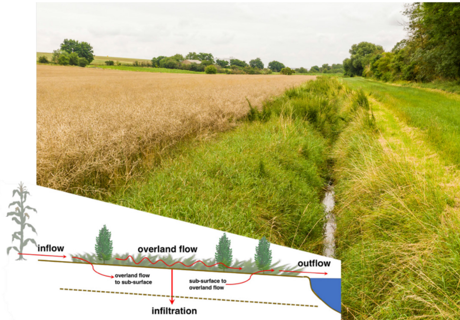
Figure 3: The pathways of pesticides and nutrients from treated agricultural fields through vegetated buffer strips into surface water bodies. Modified from Barfield et al. (1998) and Prosser et al. (2020). Photo by André Künzelmann.
