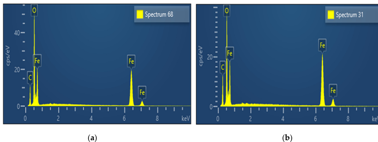
Figure 4. EDS spectrums for iron oxide particles are produced at (a) 700 °C and (b) 950 °C.
