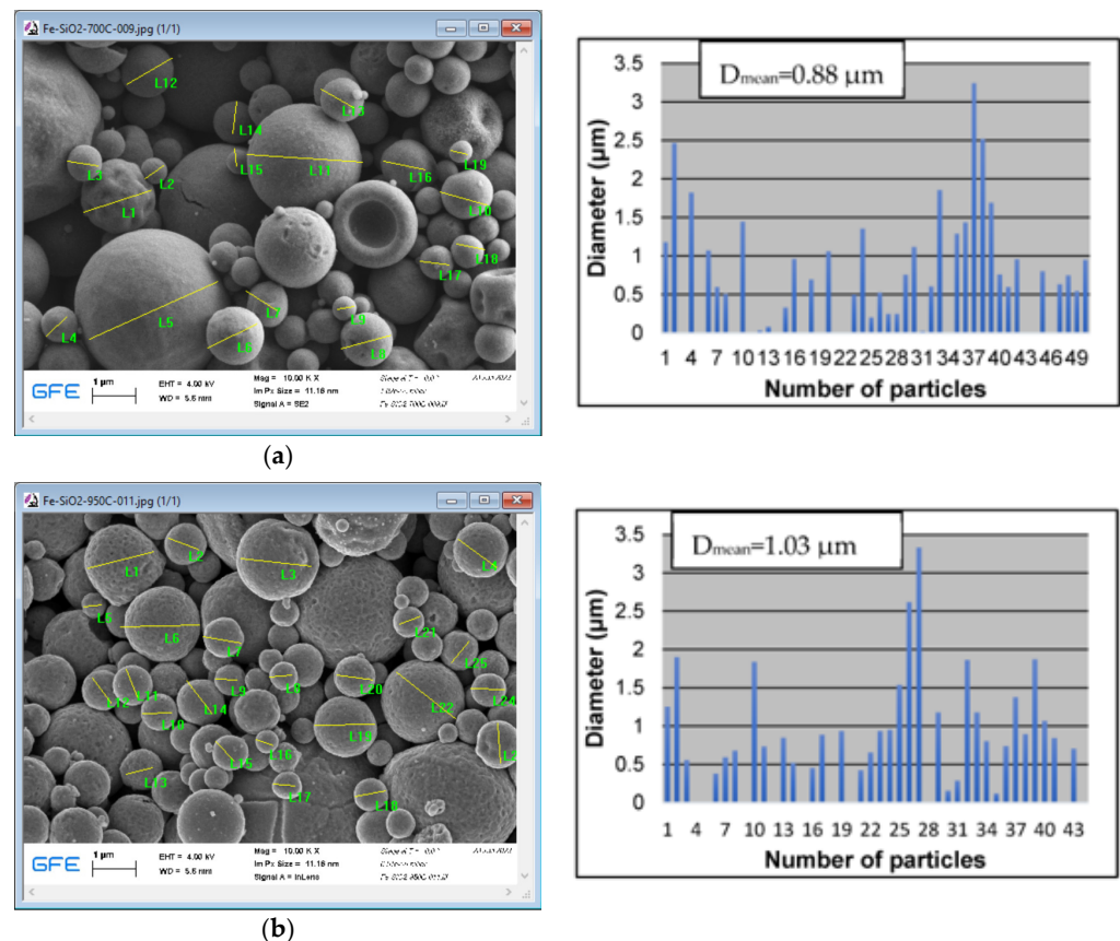
Figure 7. Mean diameters of Si-doped iron oxide particles (a) 700 °C, (b) 950 °C.
