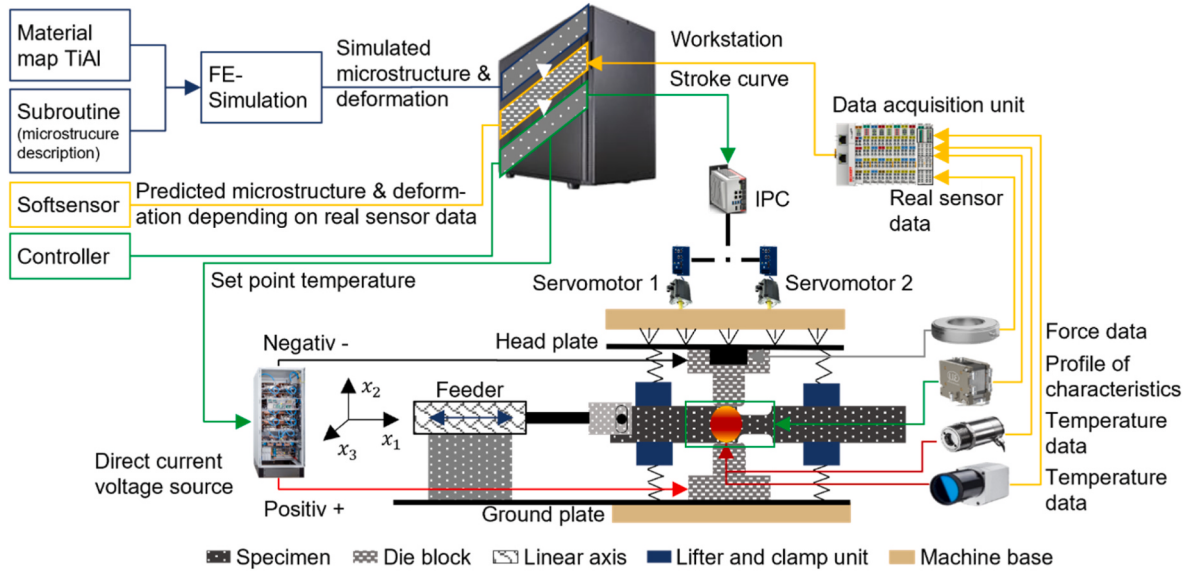
Fig. 10. Process setup and control-loop in open-die forging for local control of globularization kinetics and geometry.
