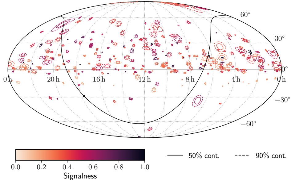
Figure 1. Skymap in Equatorial coordinates (J2000) of all neutrino candidate alerts used in the analysis described in Section 3. Contours denote the 50% (solid) and 90% (dashed) containment based on rescalings of the likelihood space according to resimulations of the event IceCube-160427A (Kankare et al. 2019, see Section 2 for more details). The color indicates the signalness of each alert event, described in the text. The Galactic Plane and Galactic Center are shown as a black solid line and dot, respectively.
