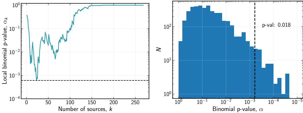
Figure 4. Binomial scan (left) and distribution of binomial p -values (right) calculated from pseudo-experiments using data scrambled in right ascension for the time-integrated analysis, as described in Section 4. In the binomial scan, the results for all alert followups is ordered by decreasing significance, and for each possible number of sources, k , we calculate the probability of obtaining k results each with p -values less than or equal to p_k . The global minimum corresponds to k = 23 and a binomial p -value of \alpha = 6.1 \times 10^{-4} (black line). The observed binomial p -value from data is shown with a black line, compared to the expected background distribution in blue, and results in an overall p -value of 1.8% for the time-integrated analysis.
