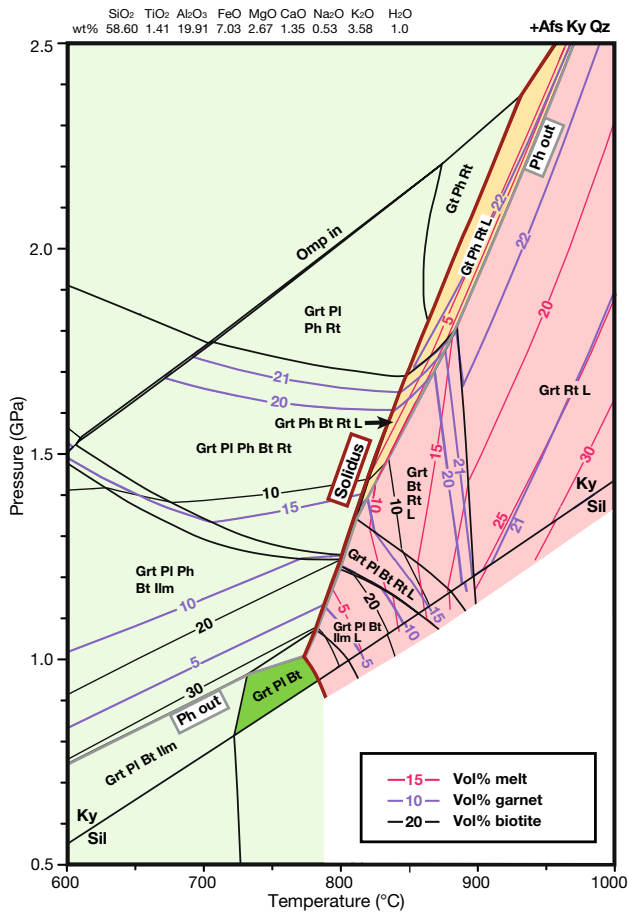
Fig. 12 Equilibrium phase diagram calculated for the metapelite T70G with an estimated content of 1 wt% H 2 O. The subsolidus stability fields are shaded in light green, the suprasolidus fields are shaded in pink. Isoleths for vol% garnet, biotite and melt are plotted. The melt volume isopleths are most dense in the narrow fields (yellow color) where phengite decomposes to form melt. At pressures below 1 GPa, the phengite-out boundary (Ph out) is very near to the kyanite-sillimanite phase boundary. The dark green field marks the stability field of the assemblage Grt + Pl + Bt + Afs + Ky + Qz present in rock matrix. Mineral abbreviations see Fig. 1
