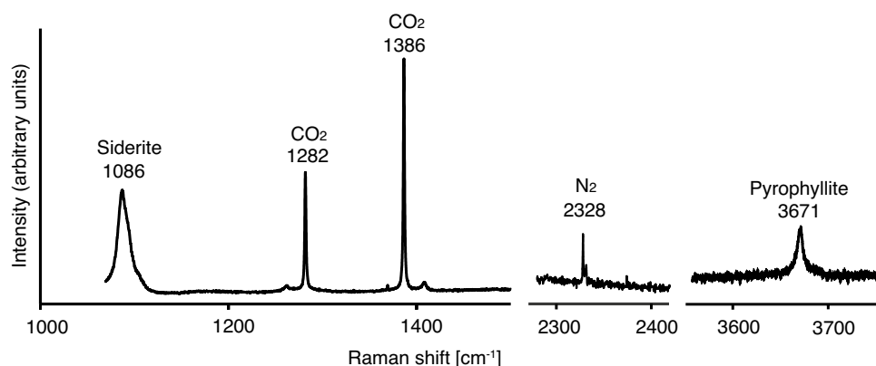
Fig. 8 a \text{CO}_2\text{-N}_2 fluid inclusions ( a , b ) with pyrophyllite ( a : \text{N}_2=0.28 mol%, \rho>1.081^* g/cm 3 ; b : \text{N}_2=0.64 mol%, \rho>1.081^* g/cm 3 ), showing similar Raman spectra (Fig. 9) but without siderite; c : dolomite with attached \text{CO}_2\text{-N}_2 fluid inclusion ( \text{N}_2=3.4 mol%, \rho=0.64 g/cm 3 ). b Fluid inclusions radiating from a decrepitated polymineralic silicate-rich inclusion. One analyzed inclusion with \text{CO}_2\text{-N}_2 ( \text{N}_2=0.76 mol%, \rho=0.84 g/cm 3 ) contains siderite and
