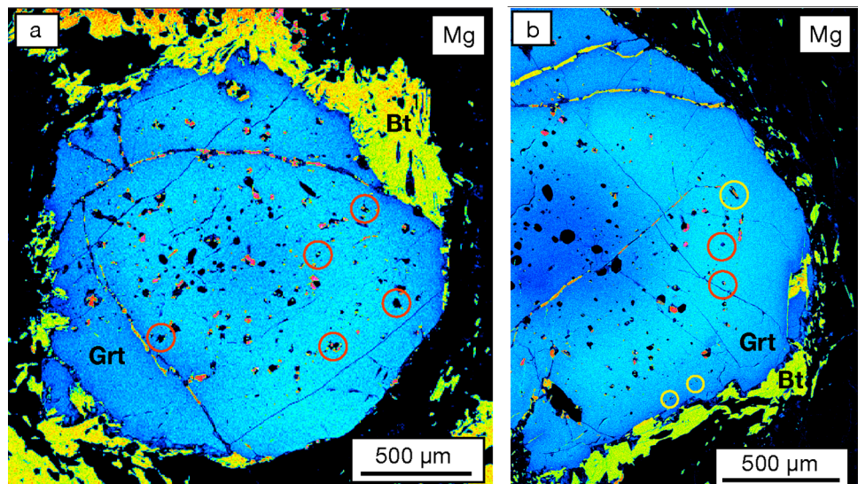
Fig. 5 EDS X-rays element distribution maps for Mg of zoned garnet porphyroblasts a, b showing the location of the silicate-rich polyminer-alic inclusions (red circles) and carbonate-rich inclusions (yellow circles); b silicate and carbonate-rich inclusions occur together in the Mg-rich growth zone. Grt garnet, Bt biotite
