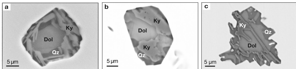
Fig. 6 BSE images of carbonate-rich polyminer-alic inclusions (Type II) in garnet. Inclusions with dolomite (> 10 vol%), quartz, kyanite show negative crystal shape a, b but also irregular shapes occur c . Dol dolomite, Qz quartz, Ky kyanite
