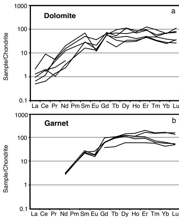
Fig. 10 a Chondrite-normalized (Boynton 1984) REE pattern of dolomite in the carbonate-rich inclusions and b of the host garnet surrounding the carbonate-rich inclusions
