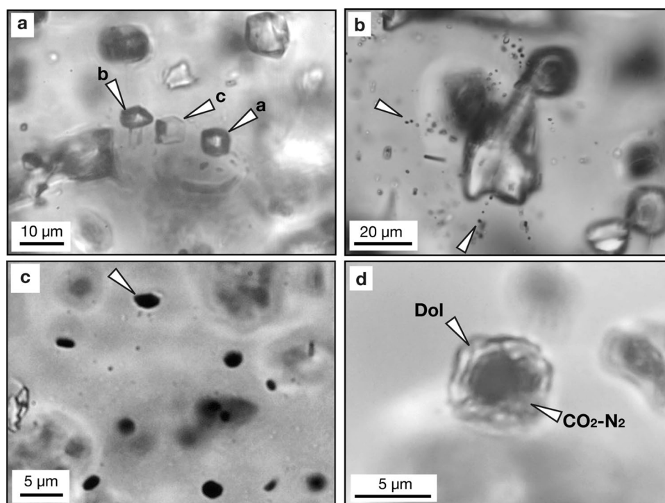
Fig. 8 a \text{CO}_2\text{-N}_2 fluid inclusions ( a , b ) with pyrophyllite ( a : \text{N}_2=0.28 mol%, \rho>1.081^* g/cm 3 ; b : \text{N}_2=0.64 mol%, \rho>1.081^* g/cm 3 ), showing similar Raman spectra (Fig. 9) but without siderite; c : dolomite with attached \text{CO}_2\text{-N}_2 fluid inclusion ( \text{N}_2=3.4 mol%, \rho=0.64 g/cm 3 ). b Fluid inclusions radiating from a decrepitated polymineralic silicate-rich inclusion. One analyzed inclusion with \text{CO}_2\text{-N}_2 ( \text{N}_2=0.76 mol%, \rho=0.84 g/cm 3 ) contains siderite and
