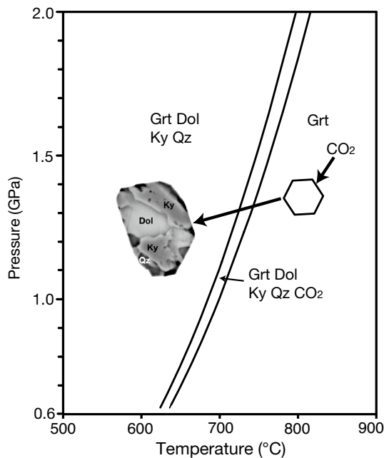
Fig. 14 Equilibrium phase diagram calculated by THERIAK-DOMINO for host garnet (Gt6: composition given in Table S1) near carbonaceous inclusions combined with \text{CO}_2 fluid (5 mol Gt6 + 1 mol \text{CO}_2 ). The mineral assemblages formed by reaction of \text{CO}_2 fluid with the garnet host after temperature decrease is displayed in a BSE image. Mineral abbreviations see Fig. 1
