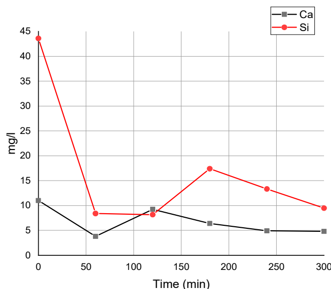
Figure 3. Change in Ca and Si concentrations over time ( T = 80^\circ\text{C} , 60–300 min).
