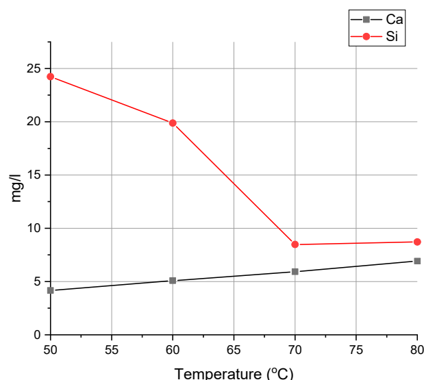
Figure 4. Change in Ca and Si concentrations for different temperatures (120 min, T = 50–80 °C).
