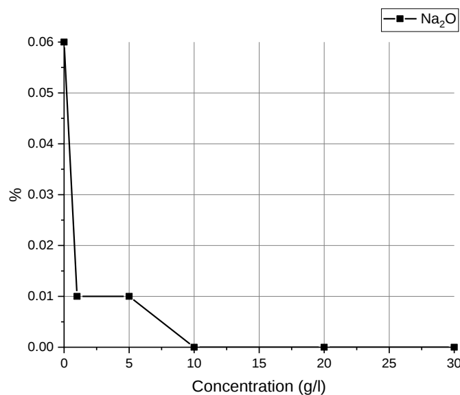
Figure 17. Effect of hydrate concentration on the reduction of sodium oxide content (210 °C, 120 min).
