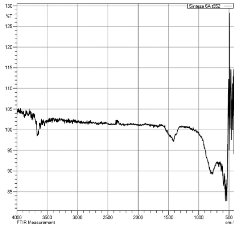
Figure 6. Infrared spectrum of the solid residue ( T = 80\text{ }^{\circ}\text{C} , 120 min, 20 g/L).
