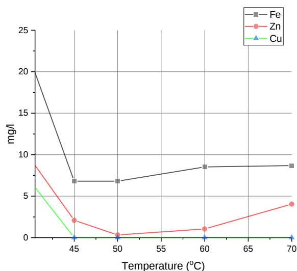
Figure 11. Changes in \text{Fe}^{2+} , \text{Zn}^{2+} , and \text{Cu}^{2+} concentrations depending on temperature (120 min, 5 g/L).
