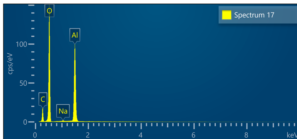
Figure 14. EDX analysis of the solid residue after the second purification step (10B: 120 min, 50 °C, 5 g/L).
