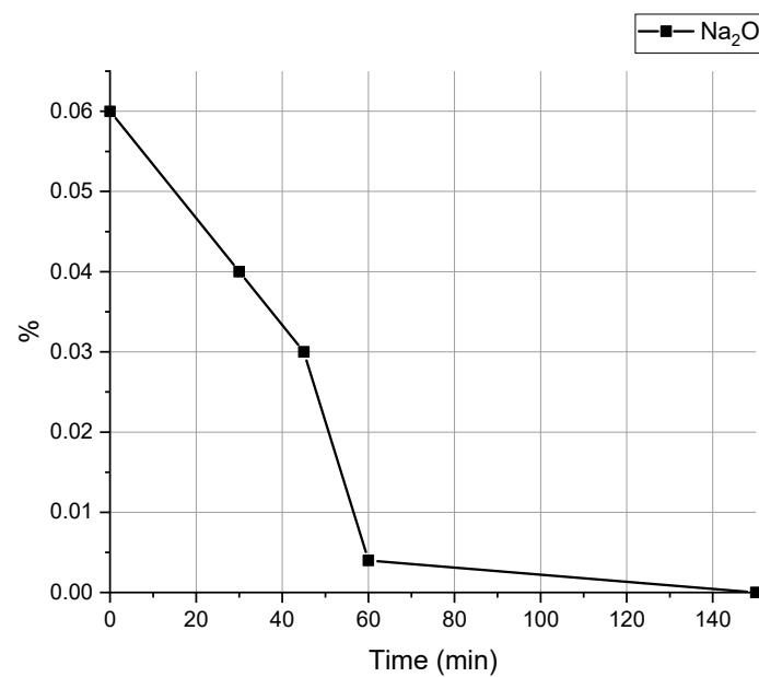
Figure 15. Effect of time on the reduction of sodium oxide concentration (210 °C, hydrate concentration of 167 g/L).
