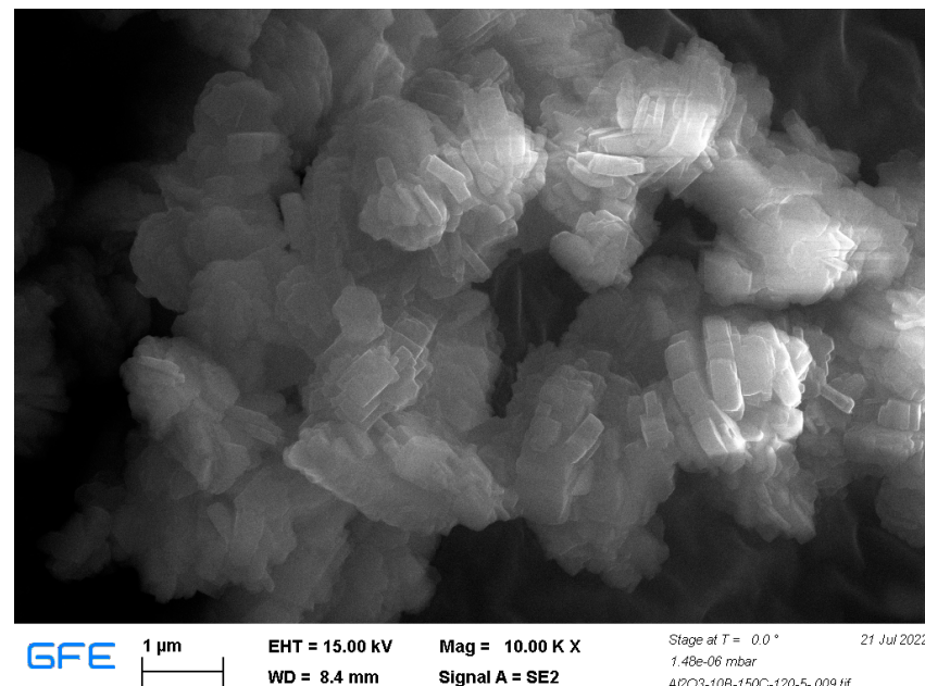
Figure 13. SEM analysis of powders after Phase II (10B: 120 min, 50 °C, 5 g/L).
