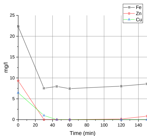
Figure 10. Changes in \text{Fe}^{2+} , \text{Zn}^{2+} , and \text{Cu}^{2+} concentrations over time ( T = 50\text{ }^{\circ}\text{C} , c = 5\text{ g/L} , t = 30\text{--}150\text{ min} ).
