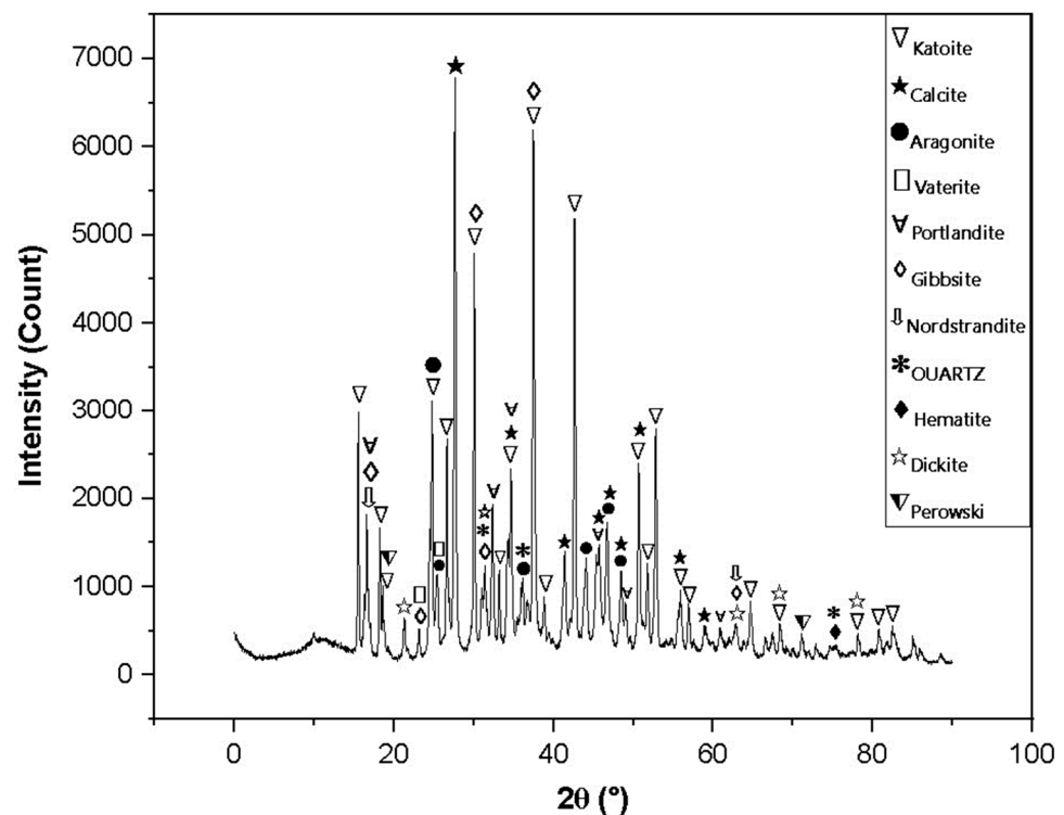
Figure 9. XRD analysis of solid residue (14A: T = 80 °C, 120 min, 40 g/L).
