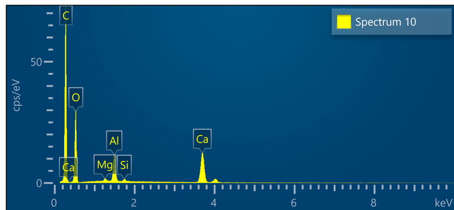
Figure 8. EDX analysis of solid residue (14A: T = 80 °C, 120 min, 40 g/L).
