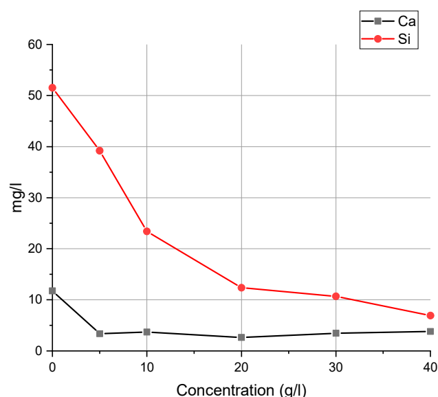
Figure 5. Influence of lime concentration on the change in Si and Ca content ( T = 80\text{ }^{\circ}\text{C} , 120 min, c = 5\text{--}40\text{ g/L} ).
