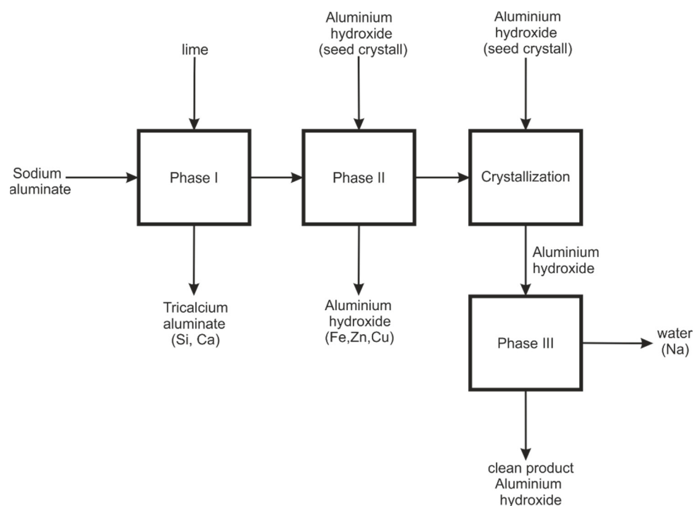
Figure 2. Schematic representation of the process.
