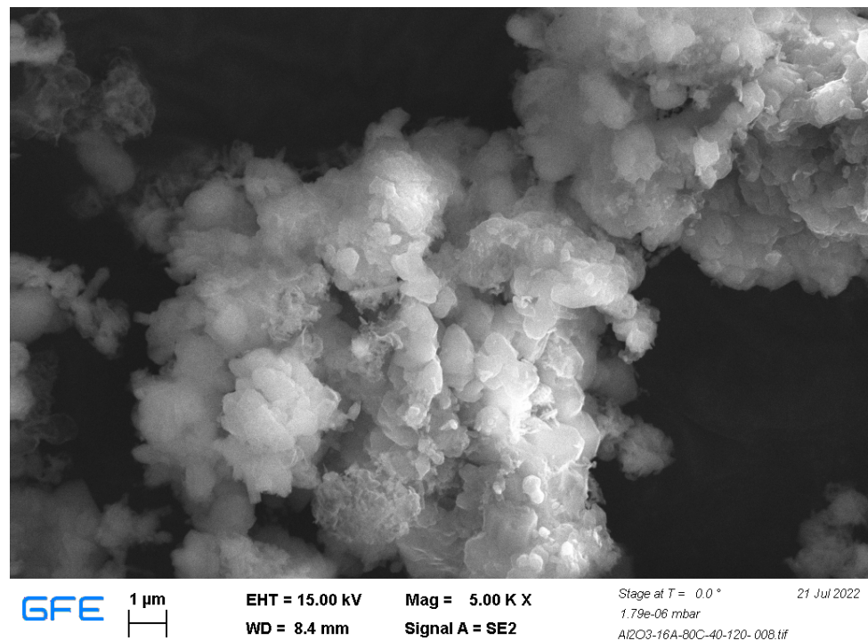
Figure 7. Typical SEM analysis of solid residue after the first purification step (14A: T = 80\text{ }^{\circ}\text{C} , 120 min, 40 g/L).
