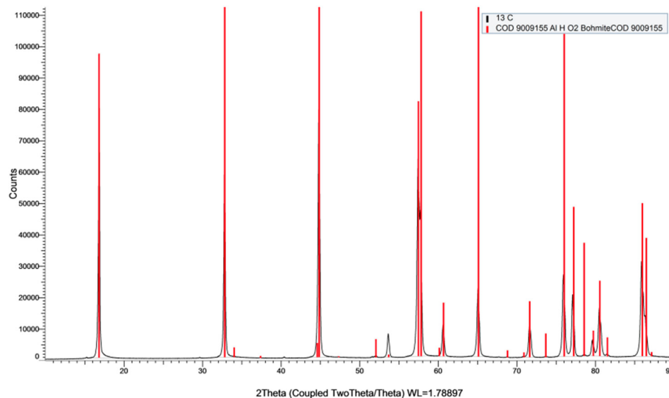
Figure 18. XRD analysis of solid product in the third purification step (210 °C, 120 min, 83 g/L).
