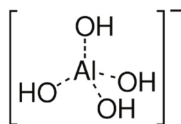
Figure 1. Structure of the aluminate ion.
