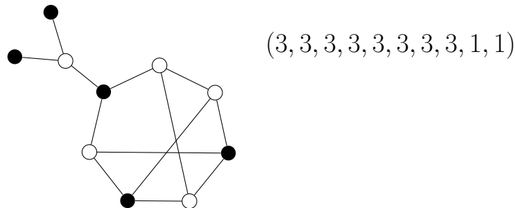
Figure 4: For k = 3 , we get n = 10 and \alpha = a = 5 \geq \frac{n}{2} , while \alpha' = 2 .
