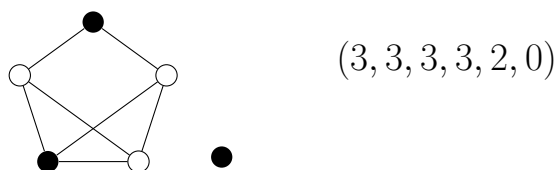
Figure 2: For a C_5 with two chords and a singleton, we obtain \alpha = a = 3 \geq \frac{n}{2} but \alpha' = 1 .
