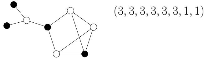
Figure 3: This graph with n = 8 fulfils \alpha = a = 4 \geq \frac{n}{2} , while \alpha' = 2 .
