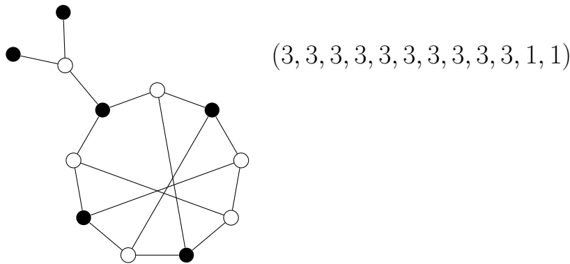
Figure 5: For k = 4 , we get n = 12 and \alpha = a = 6 \geq \frac{n}{2} , while \alpha' = 2 .
