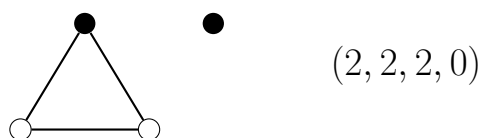
Figure 1: C_3 and a singleton with \alpha = a = 2 \geq \frac{n}{2} while \alpha' = 1 .
