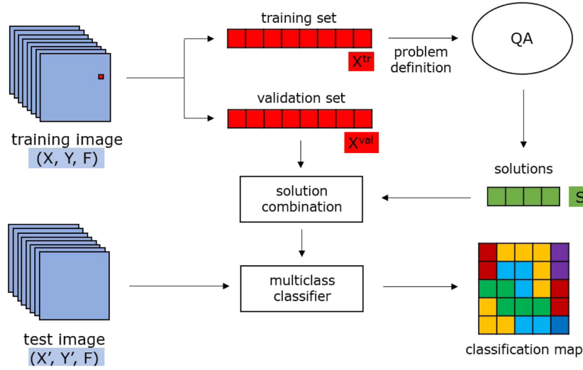
Fig. 2. Flowchart of the QMSVM algorithm. A training set X^{\text{tr}} is given as input to the QA step, which obtains a set of S solutions to the training problem. The solutions are then combined with a weighted average based on the accuracy performance on a validation set X^{\text{val}} of the classifiers obtained by the single solutions. The final classifier is then used to generate classification maps of test images.
