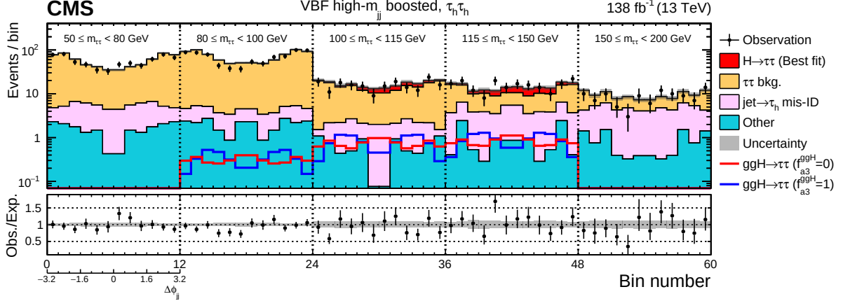
Figure 5: Observed and predicted 2D distributions after the fit to data in the VBF high- m_{jj} boosted category in the \tau_h \tau_h channel. The total H signal, including VBF, ggH, and VH processes, is shown stacked on top of the background in the solid red histogram. The ggH signal for the CP -even ( CP -odd) scenario is also shown overlaid by the red (blue) line. The uncertainty band accounts for all sources of systematic uncertainty in the signal and background predictions. The expectation in the ratio panel is the sum of the estimated backgrounds and the best fit signal.
