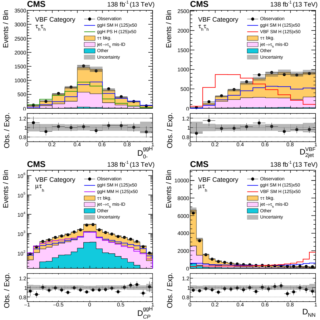
Figure 3: Examples of data and signal and background predictions for MELA and neural network discriminants in the \tau_h\tau_h and \mu\tau_h channels. Events passing the selections outlined in Sec. 6 and allocated to the VBF category are included. The yields of the H processes are scaled to match 50 times the SM predictions. The uncertainty band includes statistical uncertainties and systematic uncertainties that affect the normalization of the background distribution. The expectation in the ratio panel is the sum of the estimated backgrounds and the SM H signal. For the D_{0-}^{ggH} discriminant the distribution expected for a pseudoscalar H hypothesis (labeled “PS” in the legend) is overlaid to be compared to the SM signal. Similarly, for the D_{CP}^{ggH} discriminant the distribution for a CP-violating scenario with the maximum-mixing between CP-even and CP-odd couplings (labeled “MM” in the legend) is shown.
