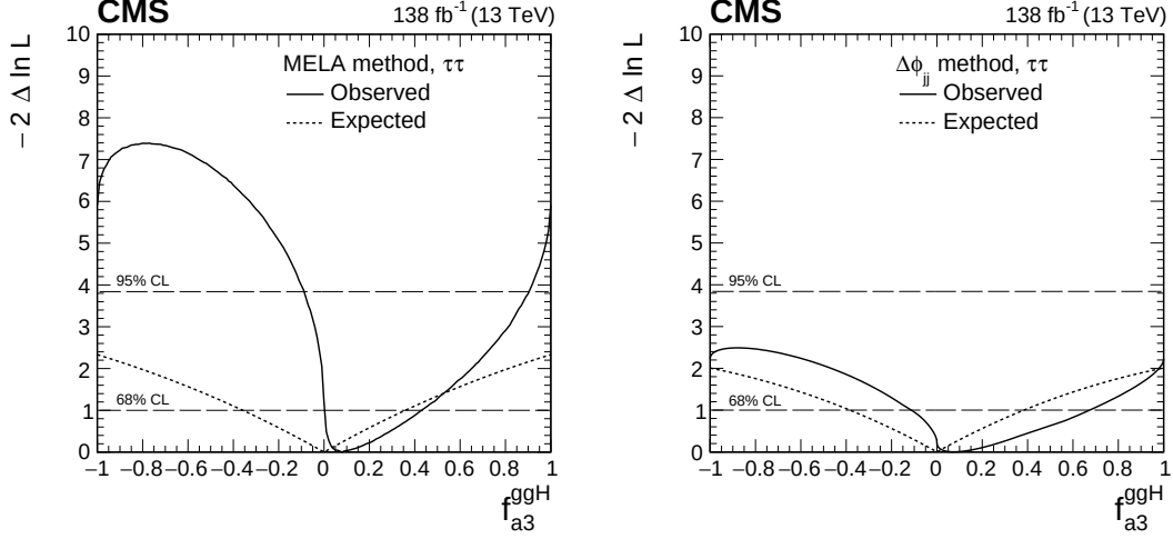
Figure 6: Observed (solid) and expected (dashed) likelihood scans of f_{a3}^{ggH} obtained with the MELA method (left) and the \Delta\phi_{jj} method used as a cross check (right).
