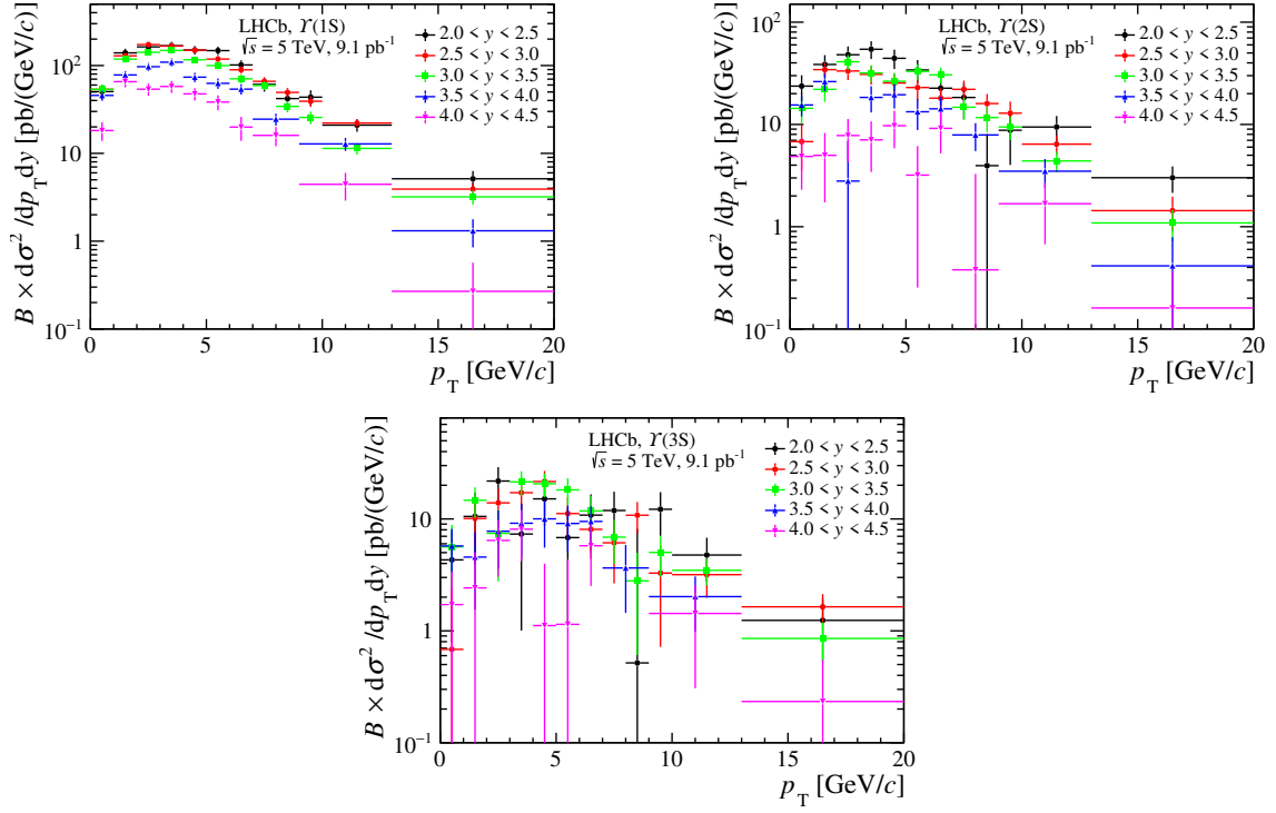
Figure 2. Double-differential cross-section times \Upsilon \rightarrow \mu^+\mu^- branching fraction as a function of p_T in bins of y for (upper left) \Upsilon(1S) , (upper right) \Upsilon(2S) and (bottom) \Upsilon(3S) mesons. Statistical and systematic uncertainties are added in quadrature.
