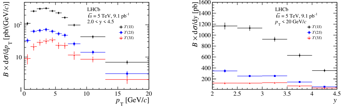
Figure 3. Differential cross-section times \Upsilon \rightarrow \mu^+\mu^- branching fraction (left) as a function of p_T for y integrated from 2.0 to 4.5 and (right) as a function of y for p_T integrated from 0 to 20 GeV/c, for the \Upsilon(1S) , \Upsilon(2S) and \Upsilon(3S) states. Statistical and systematic uncertainties are added in quadrature.
