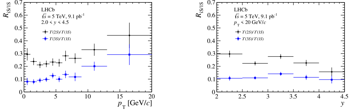
Figure 6. Ratios of the Y(2S) or Y(3S) production cross-section over that of the Y(1S) state, (left) as a function of p_T for 2.0 < y < 4.5 and (right) as a function of y for p_T < 20 GeV/c. Statistical and systematic uncertainties are added in quadrature.
