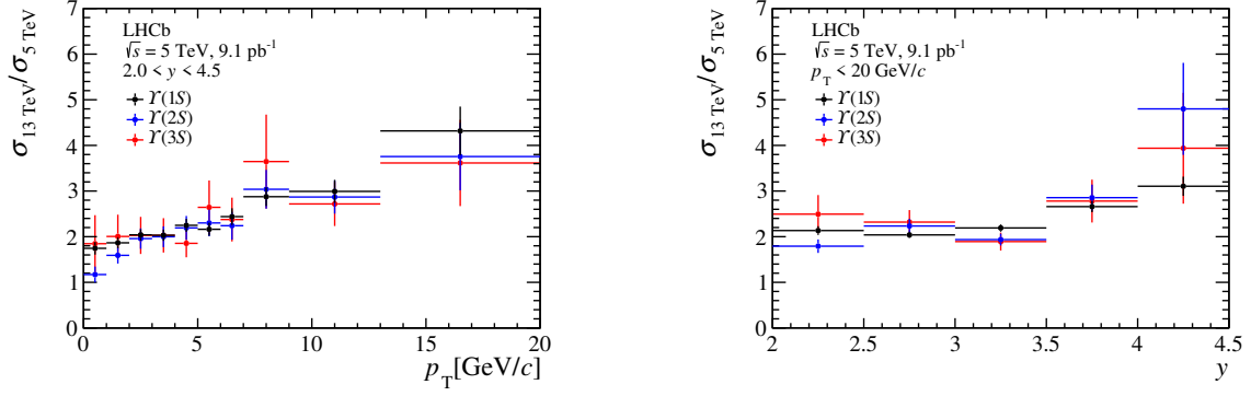
Figure 7. Ratios of \Upsilon production cross-sections measured at \sqrt{s} = 13 \text{ TeV} over those measured at \sqrt{s} = 5 \text{ TeV} (left) as a function of p_T for 2.0 < y < 4.5 and (right) as a function of y for p_T < 20 \text{ GeV}/c . The statistical and systematic uncertainties are added in quadrature.
