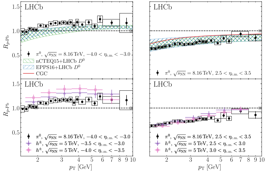
FIG. 3. Measured \pi^0 nuclear modification factor in the (left) backward and (right) forward \eta_{\text{c.m.}} regions. Error bars show the statistical uncertainty, while the open boxes show the p_T -dependent systematic uncertainties. The solid gray boxes show the overall normalization uncertainties from the luminosity estimate and efficiency correction factors. The results are compared to (top) theoretical predictions [47,49,52] and (bottom) to charged-particle data from Ref. [15]. The hatched regions show the NPQCD uncertainties of the PQCD calculations. The vertical error bars on the charged-particle results show the combined systematic and statistical uncertainties.
