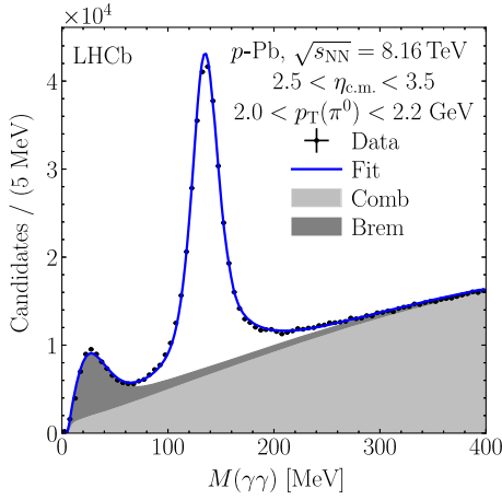
FIG. 1. Example M(\gamma\gamma) distribution in forward p -Pb collisions at \sqrt{s_{NN}} = 8.16 TeV for 2.5 < \eta_{c.m.} < 3.5 and 2.0 < p_T(\pi^0) < 2.2 GeV. Fit results are overlaid with the total fit shown as a solid line. The combinatorial (Comb) and bremsstrahlung (Brem) backgrounds are shown as light and dark shaded regions, respectively.
