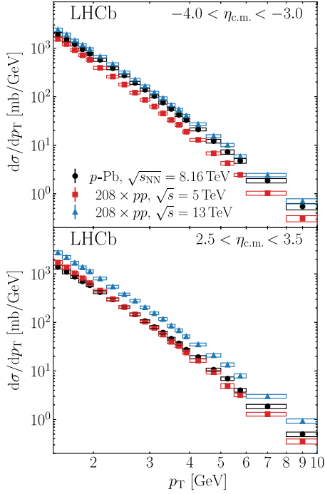
FIG. 2. Measured \pi^0 differential cross sections versus p_T in the (top) backward and (bottom) forward \eta_{\text{c.m.}} regions. Statistical uncertainties are shown by error bars, while systematic uncertainties are shown by boxes. The pp cross sections are scaled by the atomic mass of the lead ion, A = 208 .
