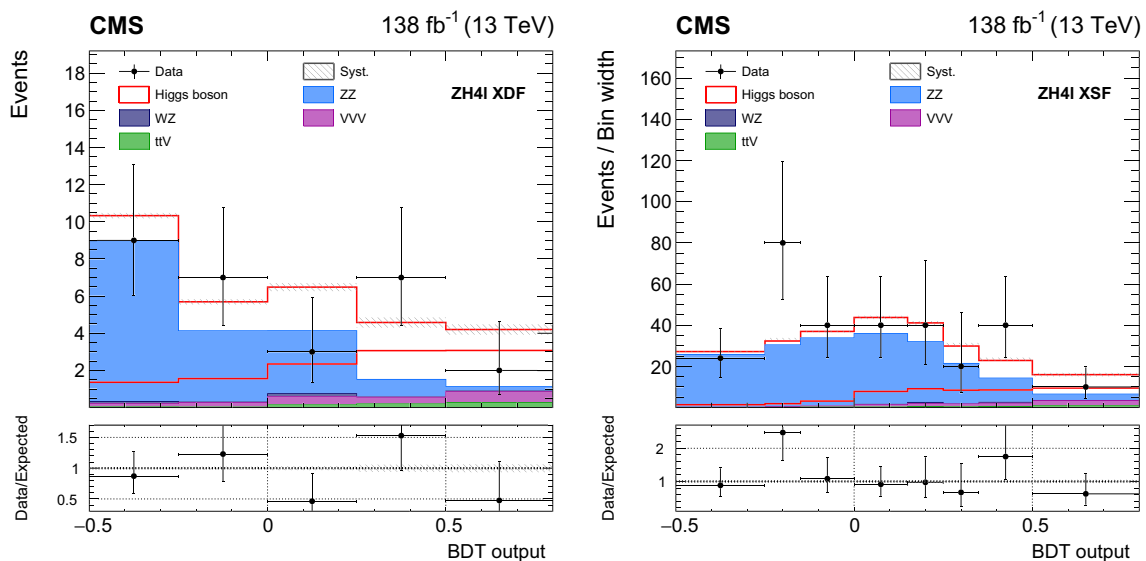
Fig. 15 Observed distributions of the BDT score in the ZH4 \ell XDF (left) and XSF (right) SRs. A detailed description is given in the Fig. 1 caption
