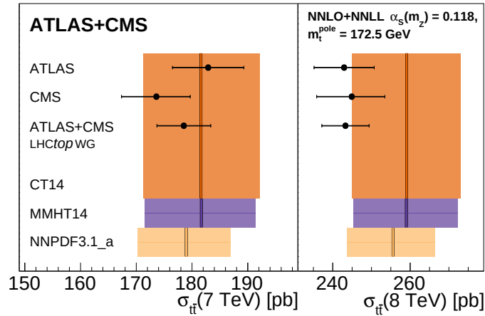
Figure 1: Measured t\bar{t} production cross-sections at \sqrt{s} = 7 and 8 TeV compared with predictions using different PDF sets. NNPDF3.1_a is a version of this PDF set containing no top-quark measurements. The shaded bands represent the total uncertainties in the predictions.
