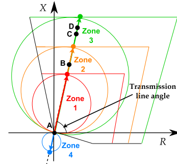
FIGURE 4. Phase and ground characteristic of the distance protection.
