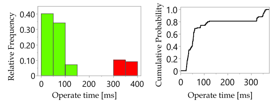
FIGURE 13. Histogram (left) and cumulative distribution plot (right) of the values of operate time for the scenario of Section VIII.
