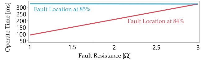
FIGURE 8. Plot of the second-order interaction between fault resistance and fault location for the three-factor scenario of Section V-A.
