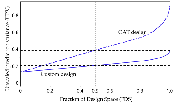
FIGURE 12. FDS plot for the custom 2^2 design and OAT design.
