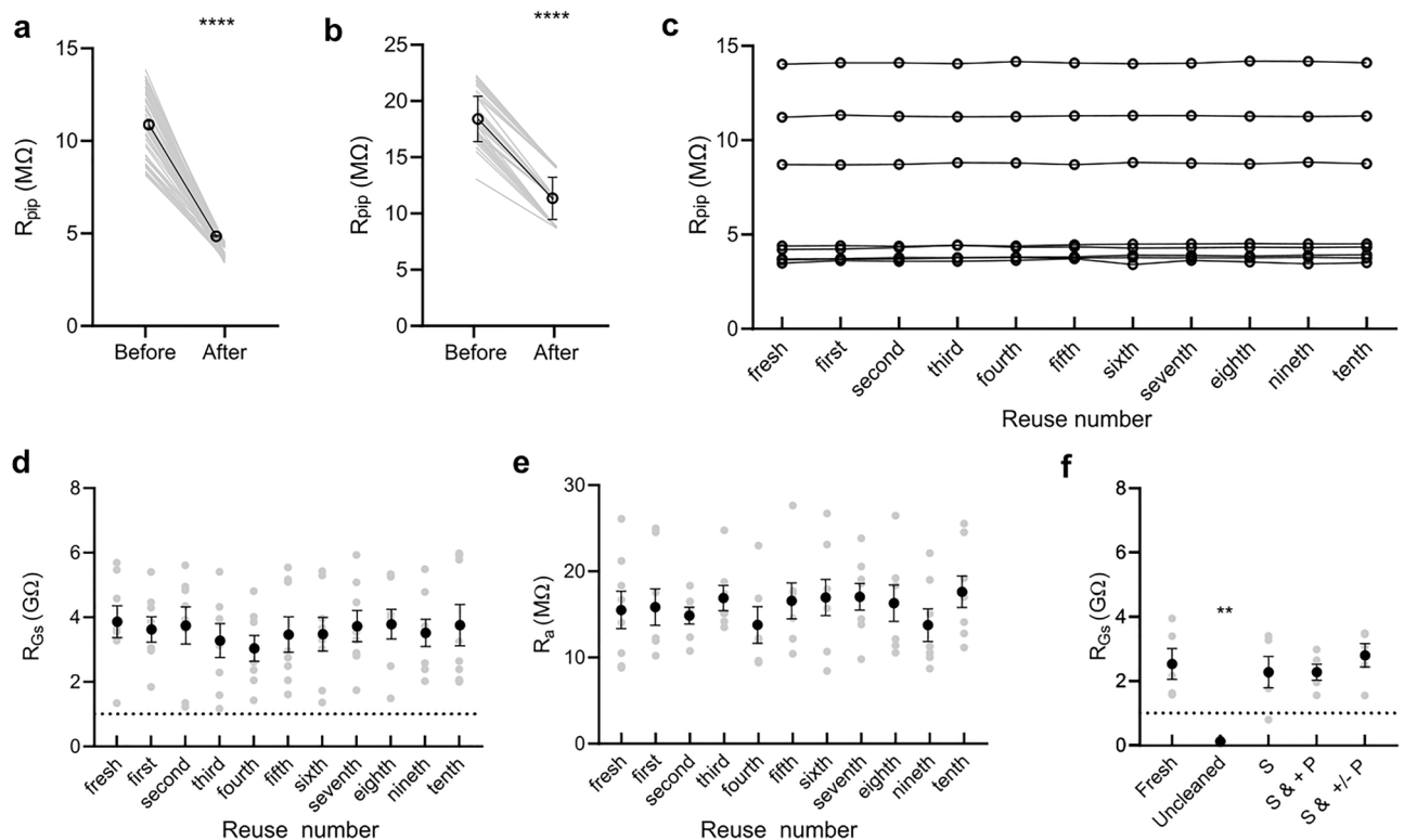
Figure 2. Ultrasonic cleaning allows reusing pipettes for multiple consecutive recordings. (a,b) Change in R_{\text{pip}} before and after cleaning of the tip of low resistance (a) and high resistance (b) pipettes. Single values are represented in grey, while mean \pm SEM values are represented in black. (c) Evolution of R_{\text{pip}} over several cleaning stages. (a–c) Ultrasonic cleaning can clean the tip as R_{\text{pip}} is recovered after each cycle. (d) Patch-clamp pipette can be successfully reused at least ten times and R_{\text{Gs}} is successfully reached. Single values are represented in grey, while mean \pm SEM values are represented in black. (e) R_{\text{a}} remains unaffected after each cleaning cycle, indicating that the tip is cleaned and the pipette can be reused for successful patch-clamp recordings. Single values are represented in grey, while mean \pm SEM values are represented in black. (f) Ultrasonic cleaning can allow pipette to be reused to reach a gigaseal. S sonification only, S & + P sonification combined with positive pressure only, S & +/– P sonification combined with alternance of positive and negative pressure.
