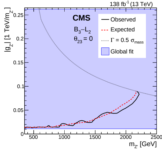
Figure 8: Exclusion limits at 95% CL in the |g_{Z'}| - m_{Z'} plane for the B_3 - L_2 model [18] for a fixed value of \theta_{23} = 0 . The solid black (dashed red) curve represents the observed (median expected) exclusion. The dotted curve denotes the coupling values at which the Z' width equals one half of the \mu\mu invariant mass resolution. For larger values of the couplings, the narrow width approximation intrinsic to the search strategy is not considered valid. The region enclosed between the solid black (dashed red) and the dotted curves is (expected to be) excluded. The shaded blue area represents the |g_{Z'}| range preferred from the global fit in Ref. [18] at 95% CL.
