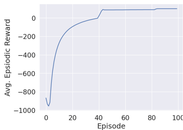
Fig. 8: The training history of the DDPG agent.
