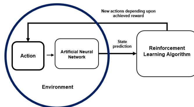
Fig. 4: The RL framework for the inverse design of silica aerogel model networks.
