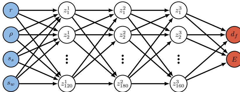
Fig. 3: Visualization of ANN network architecture with 4 inputs and 2 outputs.
