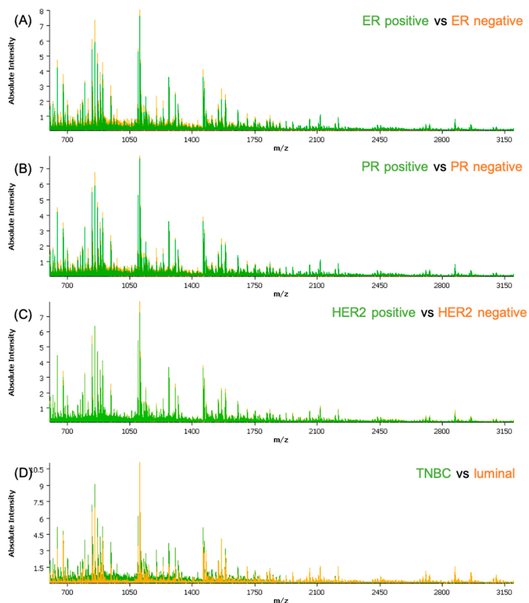
Figure 1. Comparison between the average spectra of the different classes used in the classification models: (A) ER-positive versus ER-negative; (B) PR-positive versus PR-negative; (C) HER2-positive versus HER2-negative; and (D) TNBC versus luminal. ER—estrogen receptor; PR—progesterone receptor; HER2—human epidermal growth factor receptor-2.
