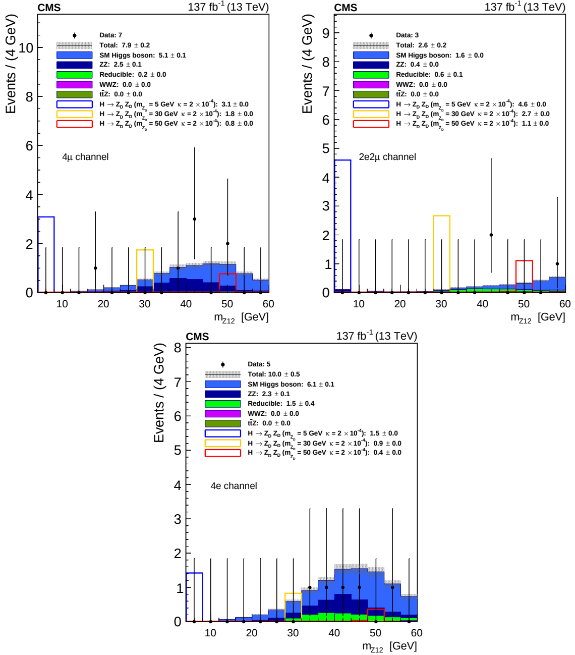
Figure 3: Event yields against m_{Z12} = (m_{Z_1} + m_{Z_2})/2 with the XX selection for the 4 \mu , 2e2 \mu and 4e final states. Numbers in the legend show the total event yields with the XX selection corresponding to data, and the expected yields for each background and signal processes, along with the corresponding statistical uncertainty coming from the amount of simulated data.
