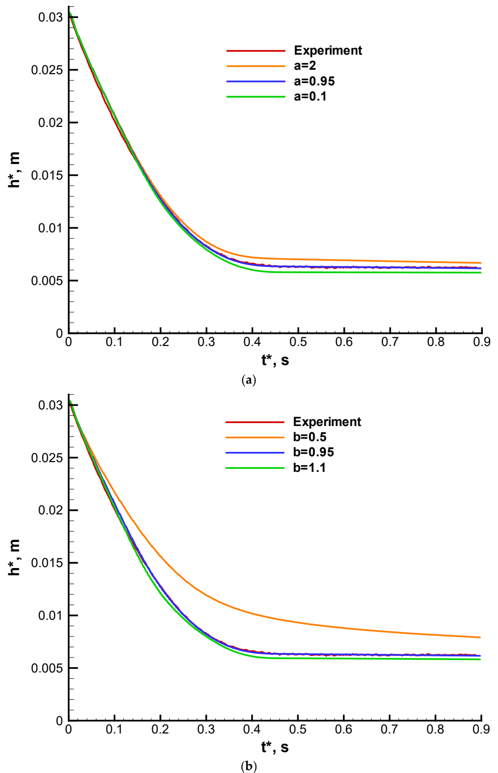
Figure 16. Effects of (a) a when b = 0.95 and (b) b when a = 0.95 and the other parameters are optimal: Re = 0.95 , Bn = 0.000235 , the power-law index varies from 0.2 to 1.4, and the initial load for the first 0.01 s is 9 kN.
