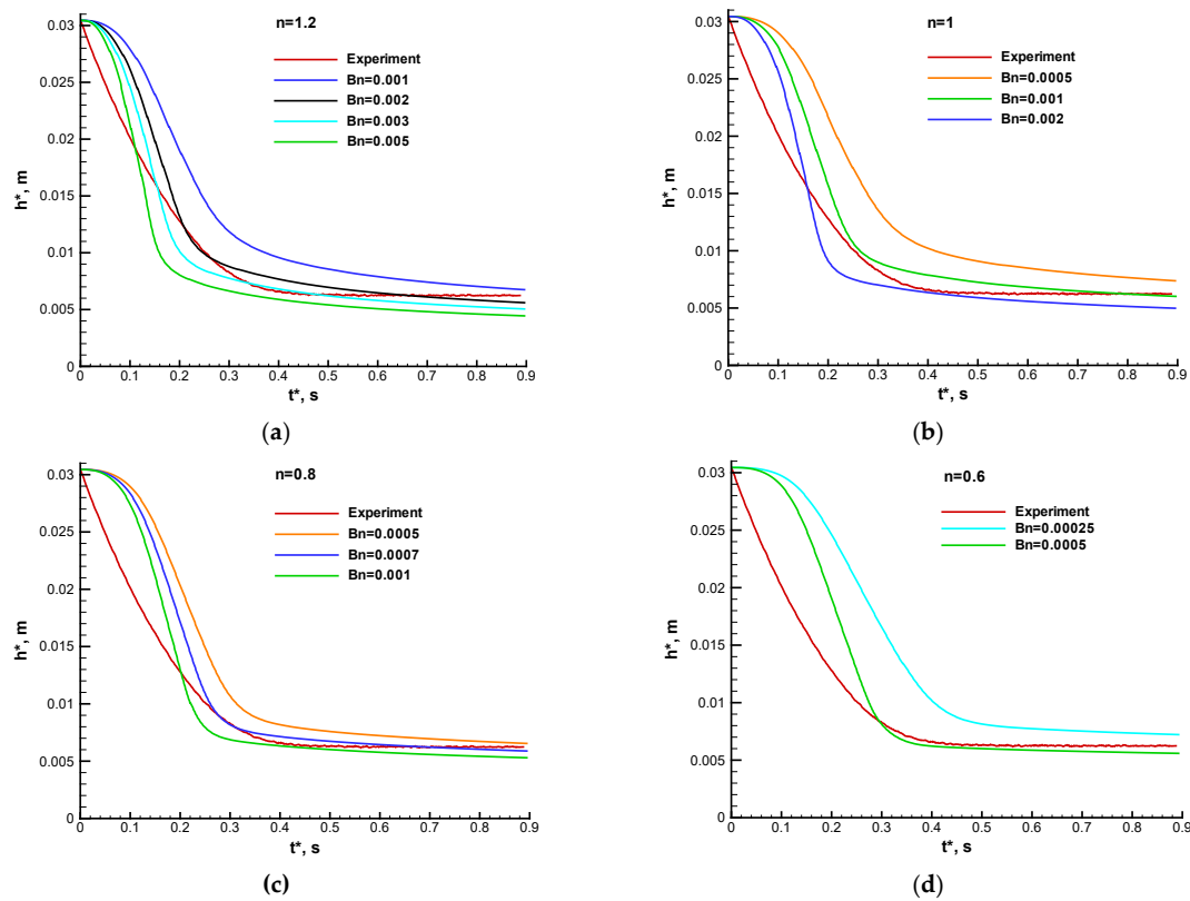
Figure 5. Effect of the Bingham number for different power-law indices when Re = 1.5 and a = b = 1 : (a) n = 1.2 ; (b) n = 1 ; (c) n = 0.8 ; (d) n = 0.6 . The experimental load distribution is imposed.
