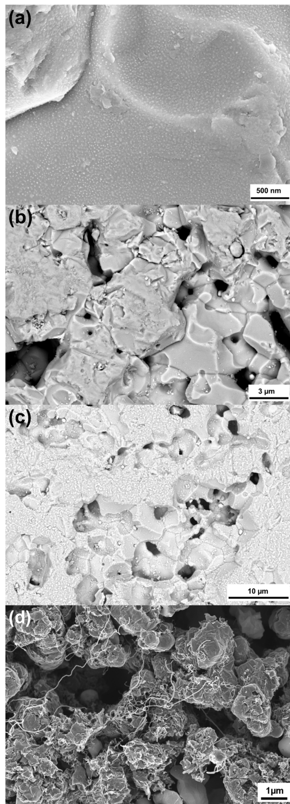
Fig. 9 SEM micrographs of (a and b) reduced (710 °C) and (c) reoxidized STF and (d) 8YSZ after carbon degradation experiments. (a and b) show SE and (b and c) show backscattered electron (BSE) micrographs.
