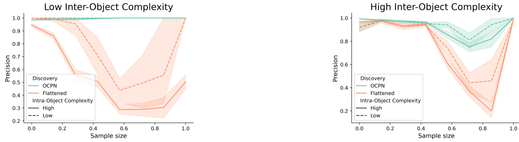
Figure 7: Discovered model precision depending on the sample size of the event log for the four different quadrants of our process taxonomy.
