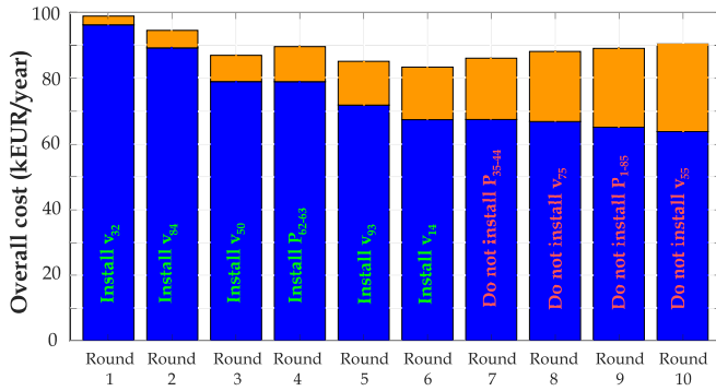
Fig. 7. Overall cost for consecutive meter placement rounds, split between redispatch costs (blue) and meter installation costs (orange).
