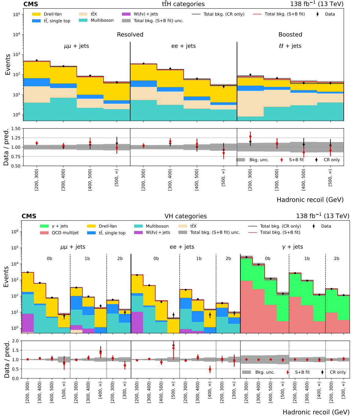
Figure 4: Distributions of hadronic recoil in the t\bar{t}H category for the \mu\mu + \text{jets} , ee + \text{jets} , and \ell\ell + \text{jets} CRs (upper plot), and the VH category for the \mu\mu + \text{jets} , ee + \text{jets} , and \gamma + \text{jets} CRs (lower plot). The black histogram shows the total background (bkg.) prediction from a CR only, B-only fit, while the red histogram shows the yields from a CR+SR S+B fit. The uncertainty in the predicted background (Bkg. unc.) accounts for both systematic and simulated statistical contributions.
