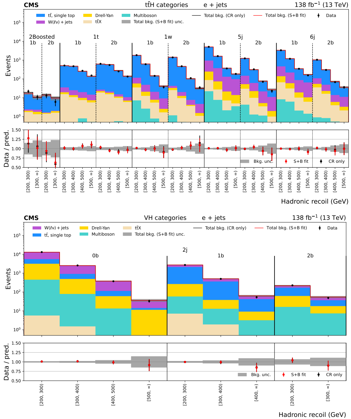
Figure 3: Distributions of hadronic recoil in the t\bar{t}H (upper plot) and VH (lower plot) categories for the e + \text{jets} CR. The black histogram shows the total background (bkg.) prediction from a CR only, B-only fit, while the red histogram shows the yields from a CR+SR S+B fit. The uncertainty in the predicted background (Bkg. unc.) accounts for both systematic and simulated statistical contributions.
