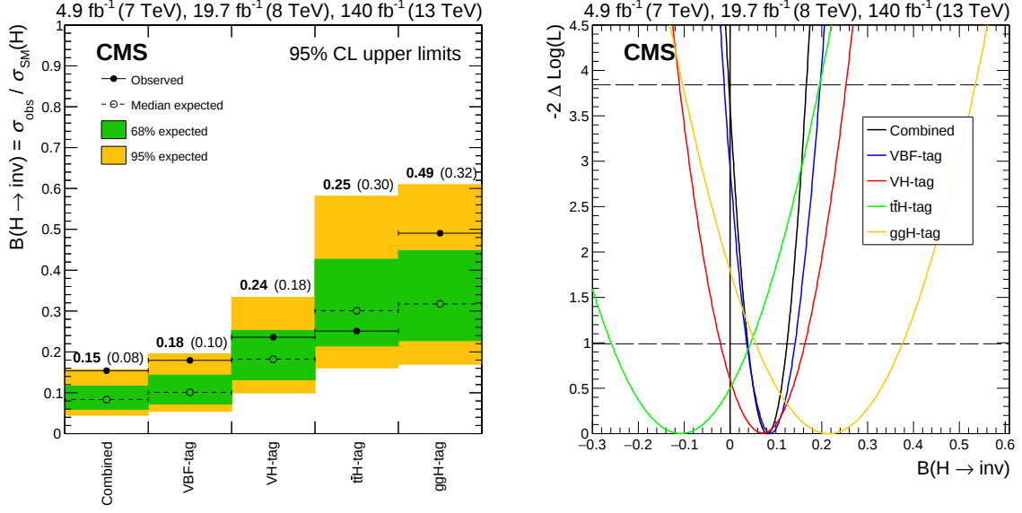
Figure 7: Left: Exclusion limits at 95% CL on B(H \rightarrow \text{inv}) . The results are shown separately for each Higgs boson production mode as tagged by the input analyses for Run 1 and Run 2, as well as combined across modes. Right: Scan of the profile negative log-likelihood as a function of B(H \rightarrow \text{inv}) broken down by the Higgs boson production mode as tagged by the input analyses for Run 1 and Run 2.
