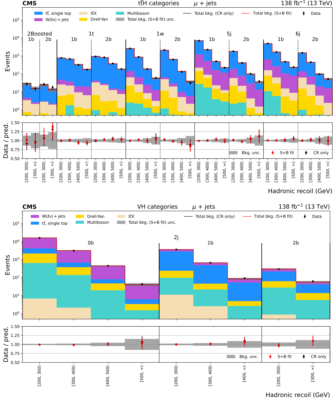
Figure 2: Distributions of hadronic recoil in the t\bar{t}H (upper plot) and VH (lower plot) categories for the \mu + \text{jets} CR. The black histogram shows the total background (bkg.) prediction from a CR only, B-only fit, while the red histogram shows the yields from a CR+SR S+B fit. The uncertainty in the predicted background (Bkg. unc.) accounts for both systematic and simulated statistical contributions.
