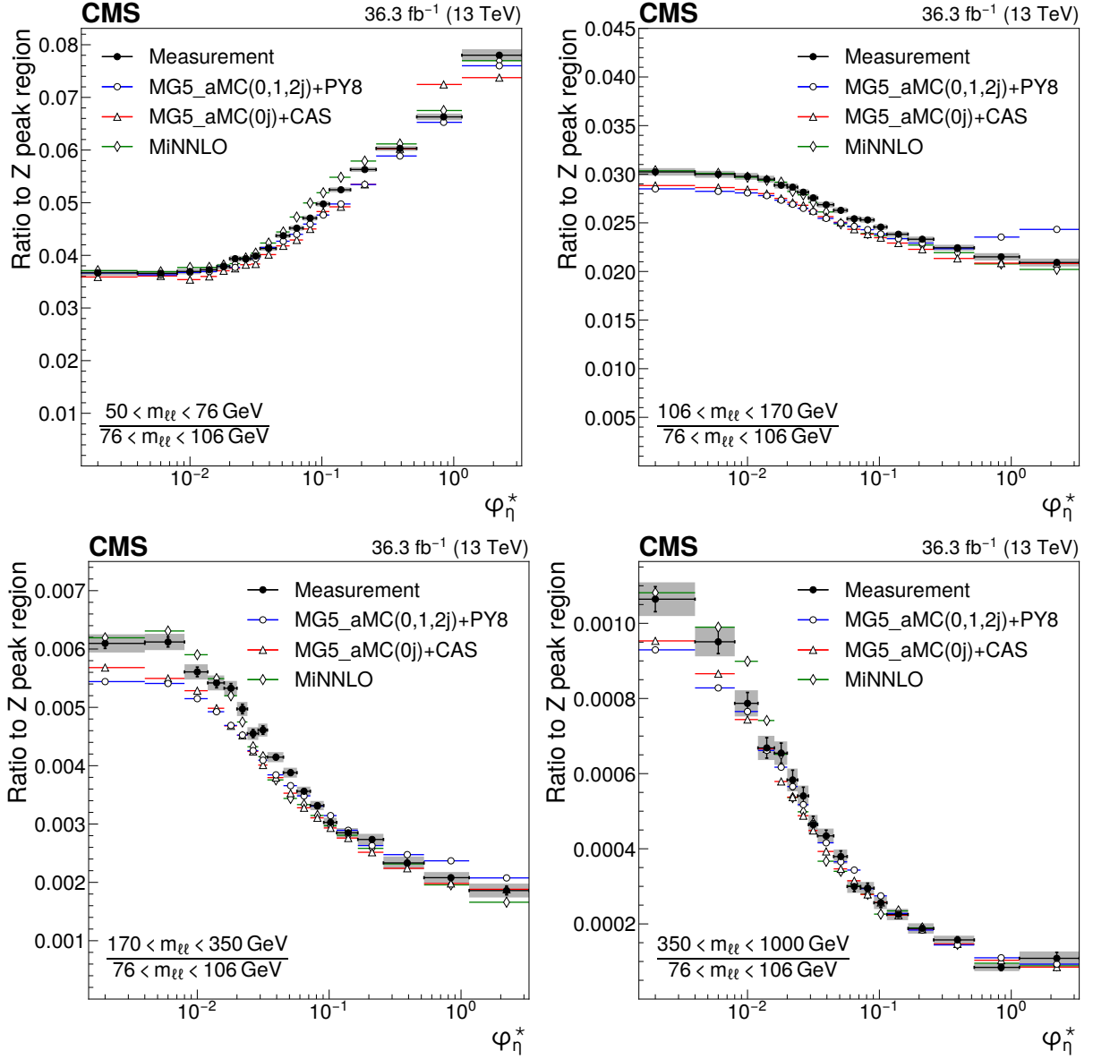
Figure 22: Ratios of differential cross sections in \phi_{\eta}^*(\ell\ell) for invariant mass ranges with respect to the peak region 76 < m_{\ell\ell} < 106 GeV: 50 < m_{\ell\ell} < 76 GeV (upper left), 106 < m_{\ell\ell} < 170 GeV (upper right), 170 < m_{\ell\ell} < 350 GeV (lower left), and 350 < m_{\ell\ell} < 1000 GeV (lower right). The measurement is compared with MG5_aMC (0, 1, and 2 jets at NLO) + PYTHIA 8 (blue dots), MiNNLO PS (green diamonds) and MG5_aMC (0 jet at NLO)+ PB (CASCADE) (red triangles). Details on the presentation of the results are given in Fig. 5 caption.
