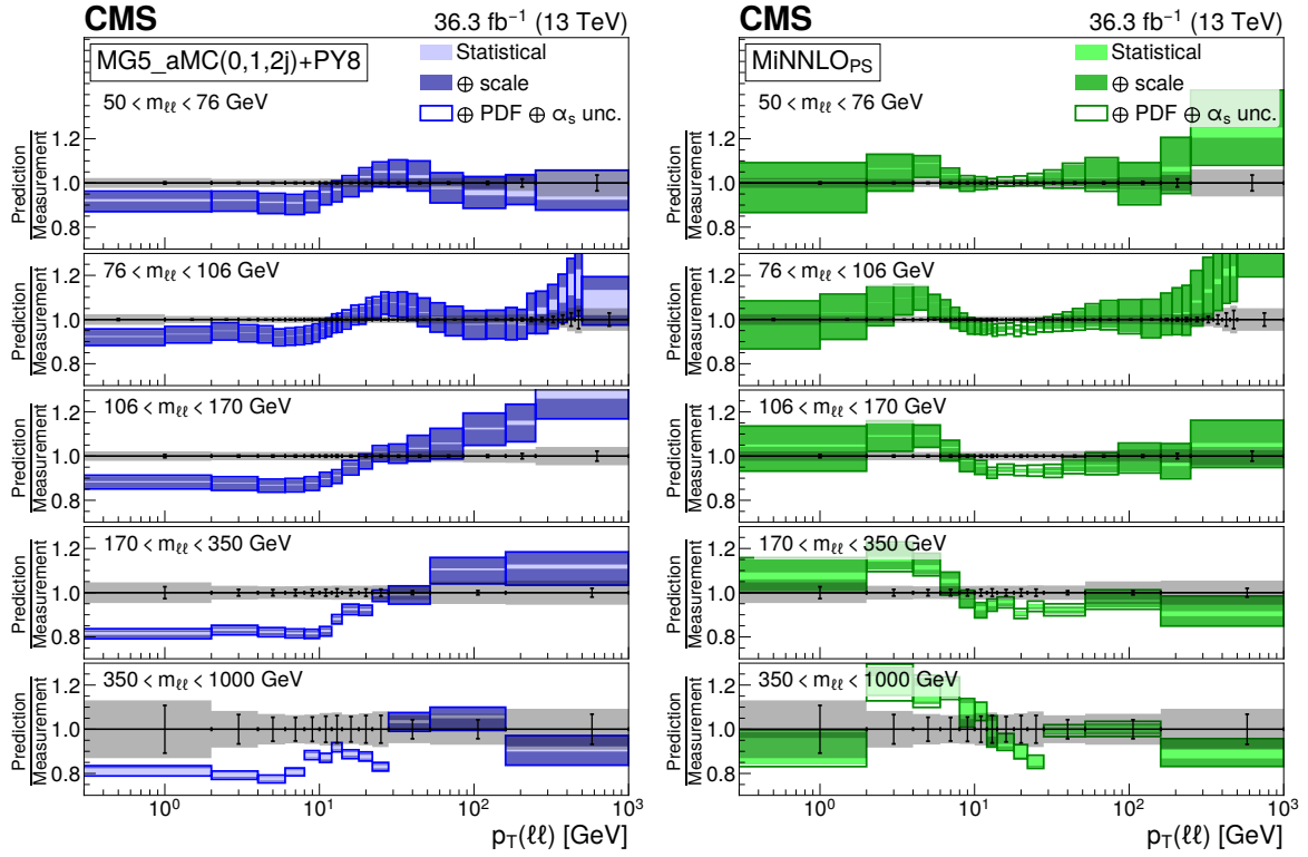
Figure 6: Comparison to Monte Carlo predictions based on a matrix element with parton shower merging. The ratio of MG5_aMC (0, 1, and 2 jets at NLO) + PYTHIA 8 (left) and MiNNLO PS (right) predictions to the measured differential cross sections in p_T(\ell\ell) are presented for various m_{\ell\ell} ranges. The error bars correspond to the statistical uncertainty of the measurement and the shaded bands to the total experimental uncertainty. The light color band corresponds to the statistical uncertainty of the simulation and the dark color band includes the scale uncertainty. The largest bands include PDF and \alpha_s uncertainties, added in quadrature.
