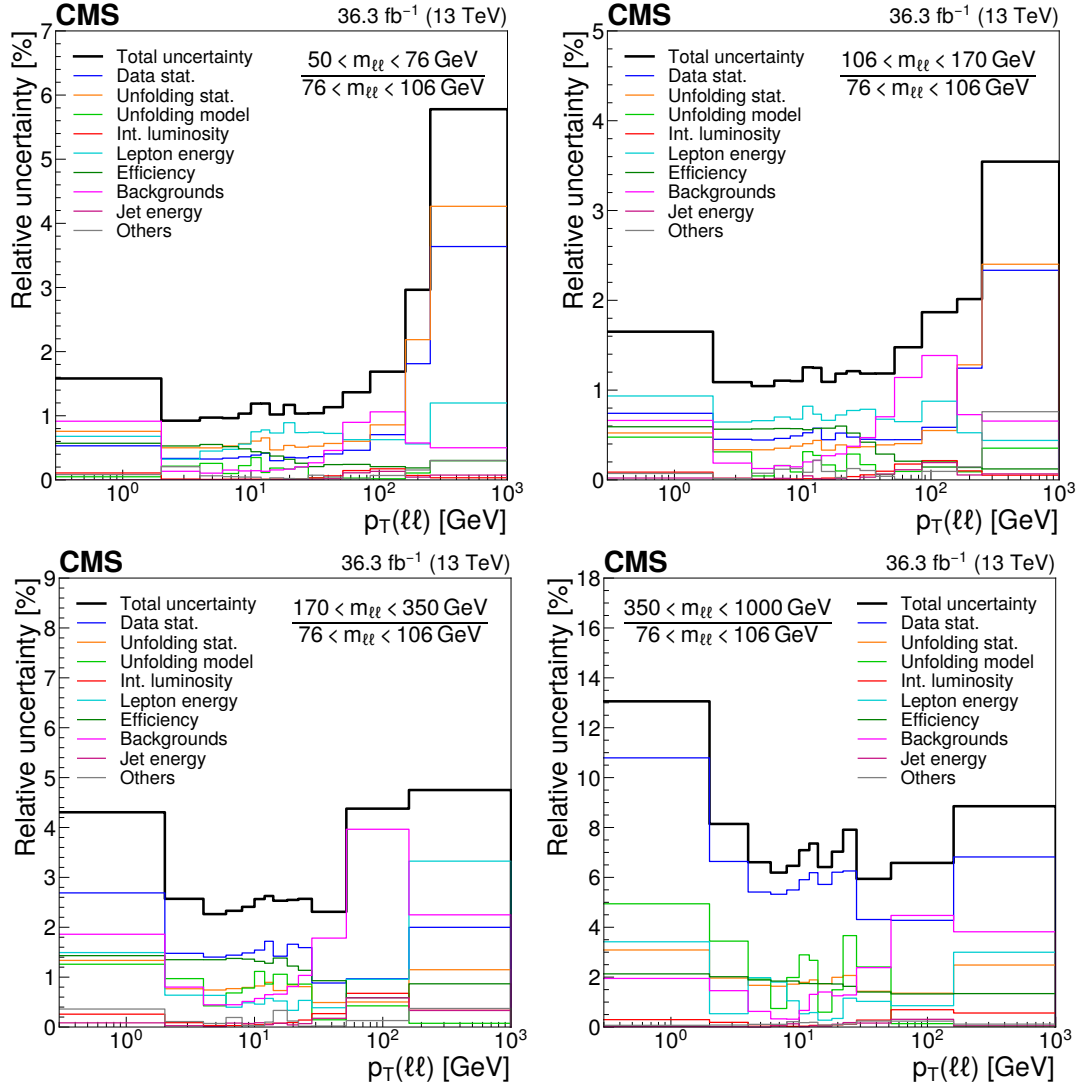
Figure 4: Estimates of the uncertainties in inclusive differential cross section ratios in p_T(\ell\ell) for invariant mass ranges with respect to the peak region 76 < m_{\ell\ell} < 106 GeV: 50 < m_{\ell\ell} < 76 GeV (upper left), 106 < m_{\ell\ell} < 170 GeV (upper right), 170 < m_{\ell\ell} < 350 GeV (lower left), and 350 < m_{\ell\ell} < 1000 GeV (lower right). The black line is the quadratic sum of the colored lines.
