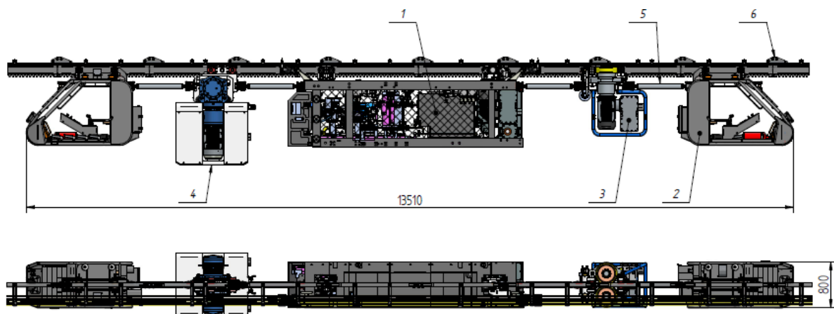
Fig. 9. SML visualization [2]
