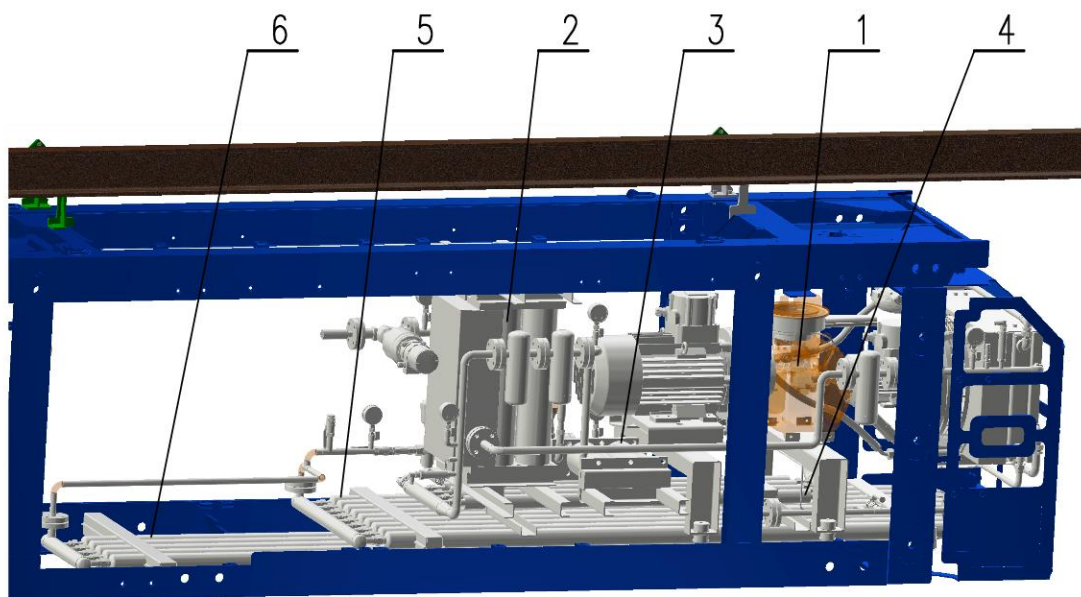
Fig. 1. Nitrogen generator visualization: (1) compressor, (2) air treatment unit, (3) carbon filters, (4) nitrogen membranes, (5, 6) two levels of tubular buffer nitrogen tanks
