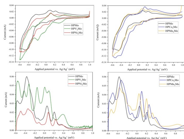
Figure 1. CV data (top left and right) of all investigated POM structures in comparison with the unsubstituted Keggin-type structure HPMo. Additionally, SWV measurements (bottom left and right) were performed to highlight the differences in the electrochemical data of the different POMs. All measurements were performed in aqueous solution at pH 1 (1 mmol/L). 0.1 M hydrochloric acid was used as supporting electrolyte.
