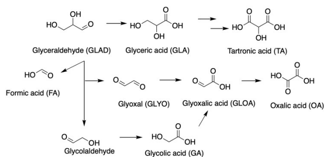
Scheme 1. Proposed reaction pathways of Keggin-type POM mediated electrolysis of GLAD.
