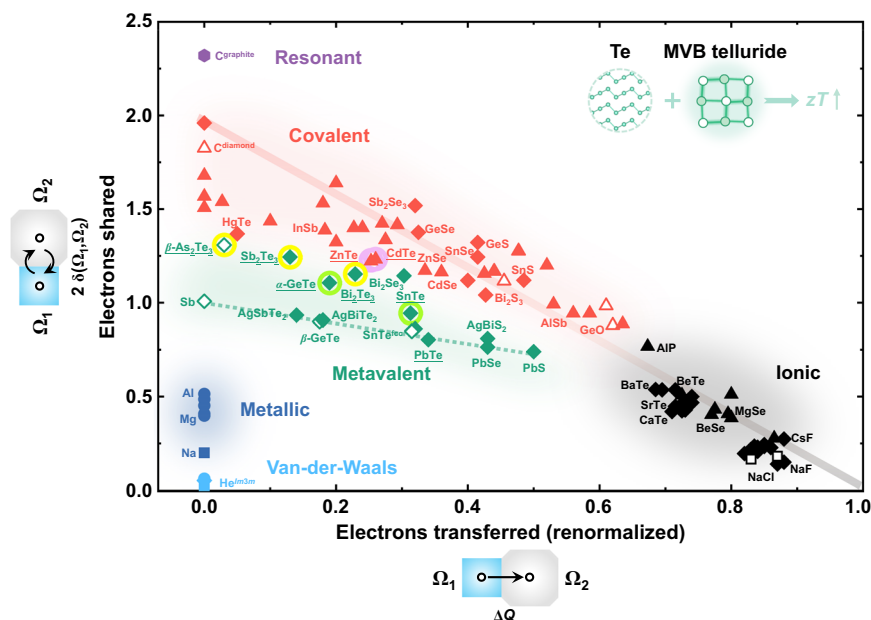
Fig. 7 | 2D map classifying chemical bonding in solids. The map is spanned by the renormalized electron transfer (ET) obtained after division through the formal oxidation state (x-axis) and the sharing of electrons (ES) between adjacent atoms (y-axis). Different colors indicate different material properties and have been related to different chemical bonding mechanisms. Ionic bonding (black-shaded area) is characterized by a significant electron transfer with an ET value larger than 0.6. In covalent solids (red-shaded area), on the contrary, there is only modest ET between atoms, but up to one electron pair (i.e., two electrons) defined by Lewis 54 are shared between neighboring atoms. Metallic bonding (blue-shaded area) is recognized by the delocalization of electrons over several neighbors and, thereby, is characterized via a small or vanishing ET and the sharing of far less than one electron between
