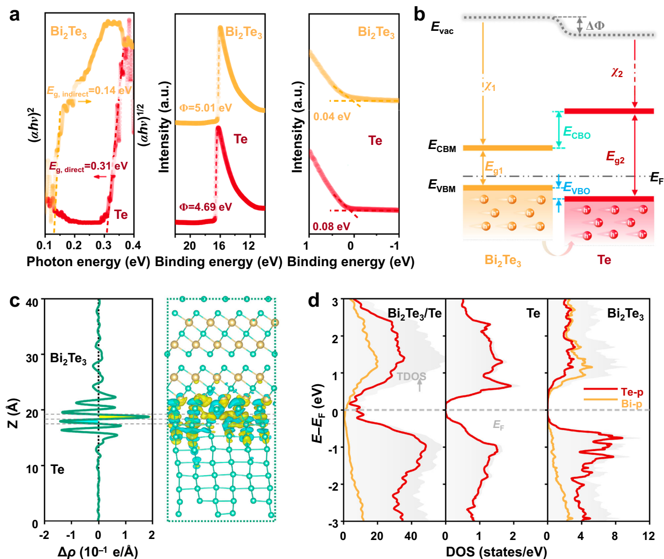
Fig. 6 | Electrical characteristics of the Bi 2 Te 3 /Te interface. a Optical bandgap, work functions, and valence band maximum (VBM) levels of Bi 2 Te 3 and Te. The band gap values were determined from Tauc plots of optical absorption coefficient (\alpha h\nu)^{1/n} versus photon energy h\nu ( h is the Planck constant and \nu is the frequency of the photon), using Fourier transform infrared spectrometer (FTIR) measurements, where the value of n is taken to be 1/2 and 2 for indirect-gap 80–82 Bi 2 Te 3 and direct-gap 51,83 Te, respectively. The work functions and VBM positions for Bi 2 Te 3 and Te are extracted from ultraviolet photoelectron spectroscopy (UPS) spectra. b Schematic showing the experimentally determined energy-level alignment at the
