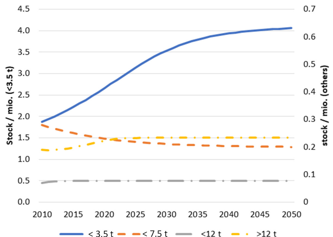
Figure 9. Calculated stock development of trucks from 2010 to 2050 divided into the weight classes of <3.5 t, <7.5 t, <12 t, and >12 t. The model is based on real stock data until 2017 taken from KBA [39].
