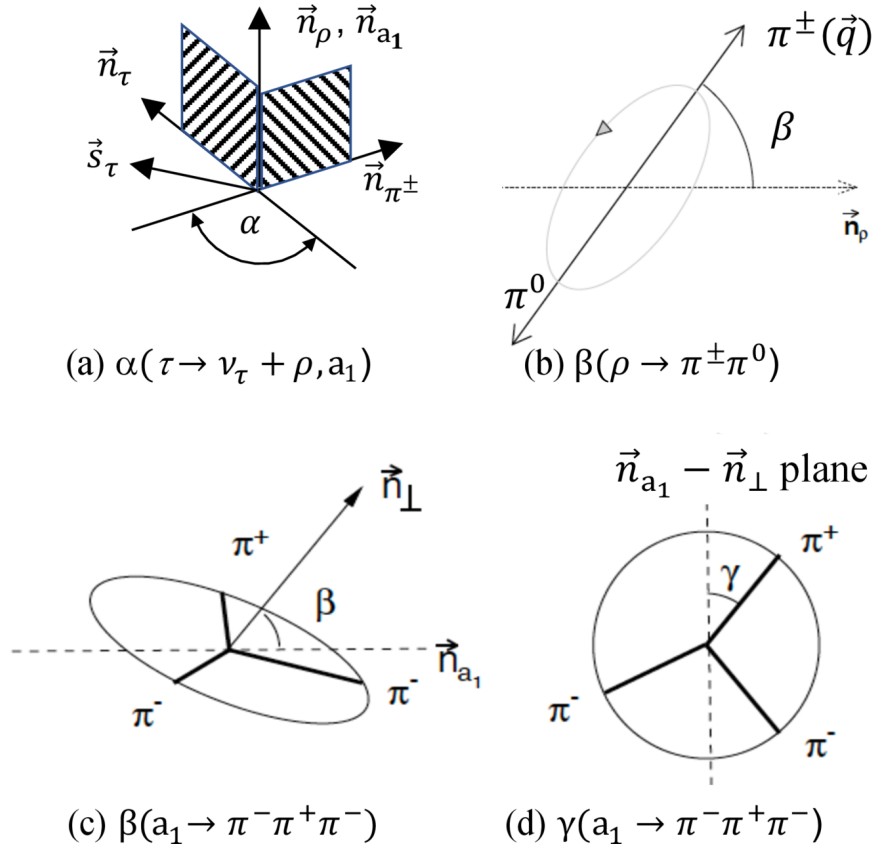
Figure 3. Definitions of (a) the angle \alpha in both \tau^- \rightarrow \rho^- \nu and \tau^- \rightarrow a_1^- \nu , (b) the angle \beta in \tau^- \rightarrow \rho^- \nu , \rho^- \rightarrow \pi^- \pi^0 and (c) in \tau^- \rightarrow a_1^- \nu , a_1^- \rightarrow \pi^- \pi^+ \pi^- , and finally (d) the angle \gamma for the decay of a_1^- \rightarrow \pi^- \pi^+ \pi^- . Figures b, c, and d have been taken and refurbished from ref. [38].
