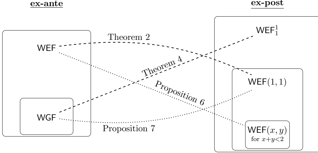
Figure 1: Summary of our results on additive valuations. Positive results are shown as dashed lines, negative results as dotted. Rectangles represent set inclusion. All our algorithms also guarantee WPROP1 ex-post.
