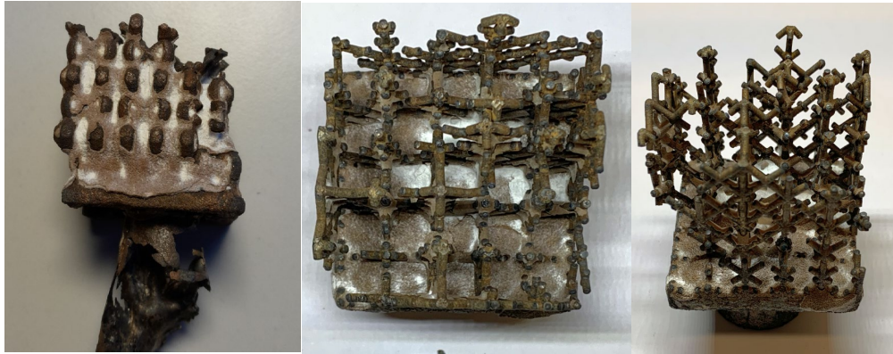
Fig. 2: Results of the first trials for casting structures with high manganese steel
