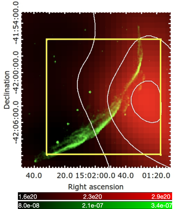
Fig. 1. Chandra flux map of SN 1006 in \text{count s}^{-1} \text{ cm}^{-2} in the 2.5–7 keV (green) band. The column density of HI in the [+5.8, +10.7] \text{ km s}^{-1} velocity range is shown in red. The contour levels of the column density at the 65%, 80% and 95% of the maximum ( 2.9 \times 10^{20} \text{ cm}^{-2} ) are shown in white. The yellow rectangle shows the NuSTAR field of view.
