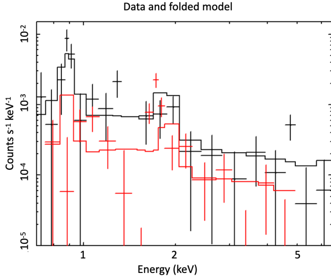
Fig. 6. XMM-Newton (EPIC-pn in black, MOS1+MOS2 in red) spectra of the knot1 with the corresponding best-fit model.
