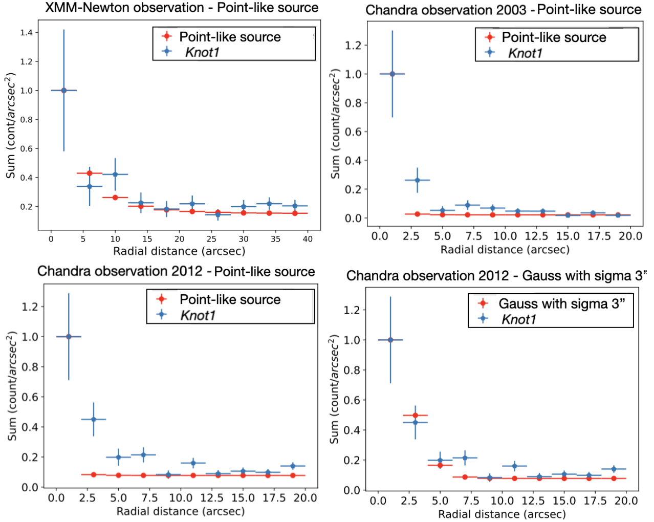
Fig. 4. Upper-left panel: comparison between the radial profiles of the knot1 surface brightness (blue crosses) and that of a simulated point-like source (red crosses, including the contribution of the background) for the XMM-Newton data. Upper-right panel: same as left panel, but for the Chandra 2003 observation. Lower-left panel: same as upper-right panel, but for the Chandra 2012 observation. Lower-right panel: same as lower-left panel, but for a simulated Gaussian profile with \sigma = 3'' (red crosses).
