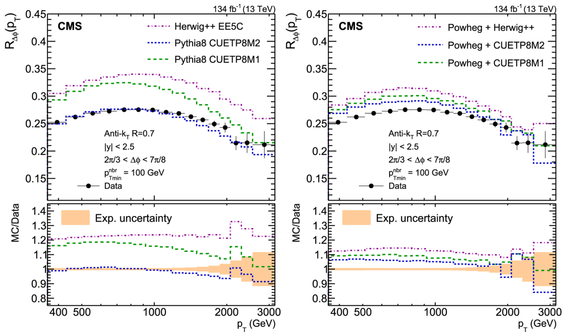
Fig. 4 The R_{\Delta\phi}(p_T) observable as a function of p_T , compared with MC generator predictions at LO (left) and at NLO (right) accuracy. The LO predictions are obtained with PYTHIA8 tunes CUETP8M1 and CUETP8M2, and HERWIG++ tune UE-EE-5-CTEQ6L1 MC event generators. The NLO predictions are obtained with POWHEG interfaced with each of the aforementioned MC event generators. The experimental data
