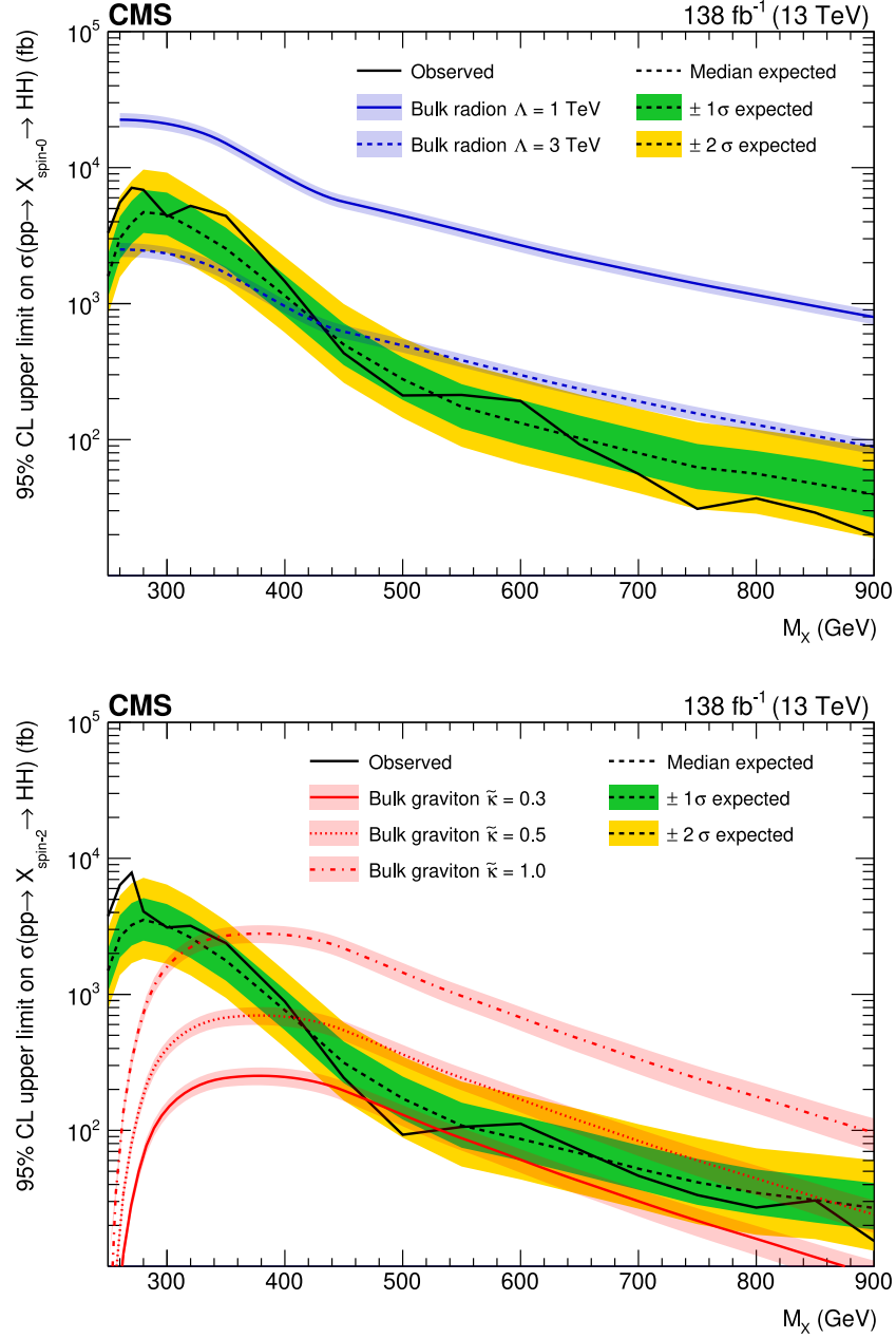
Figure 19: Observed and expected 95% CL upper limits on the production of new particles X of spin-0 (upper) and spin-2 (lower) and mass m_X in the range 250 \leq m_X \leq 900 \text{ GeV} , which decay to Higgs boson pairs. The green and yellow bands show the 1 and 2\sigma confidence intervals, corresponding to 68 and 95% CL. Theory predictions in benchmark scenarios for bulk radion (upper) and bulk graviton (lower) models are overlaid.
