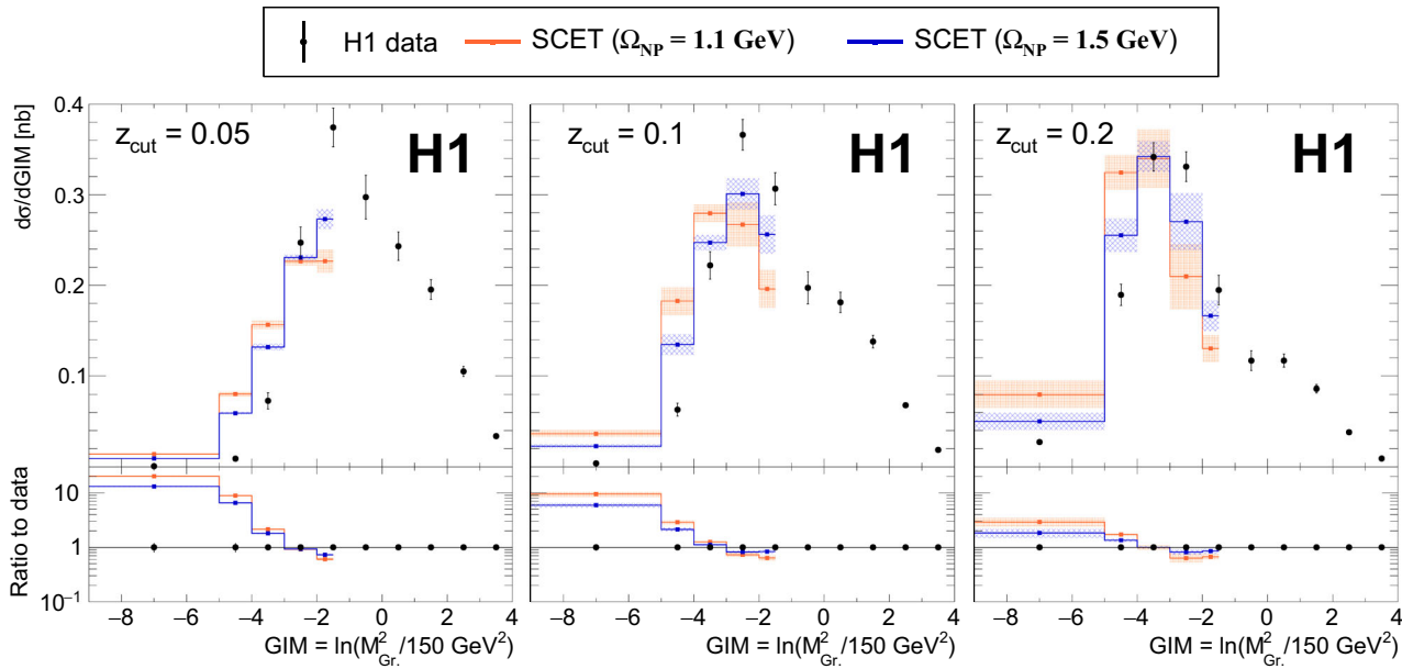
Fig. 4 Differential cross section of groomed invariant mass GIM = \ln(M_{Gr}^2/150 \text{ GeV}^2) in ep DIS at \sqrt{s} = 319 \text{ GeV} , for z_{cut} = 0.05, 0.1 and 0.2 . The value of Q_{min}^2 is set to 150 \text{ GeV}^2 . The phase space is restricted to Q^2 > 150 \text{ GeV}^2 and 0.2 < y < 0.7 . Uncertainty bars on the data show the quadrature sum of the statistical error and sys-
