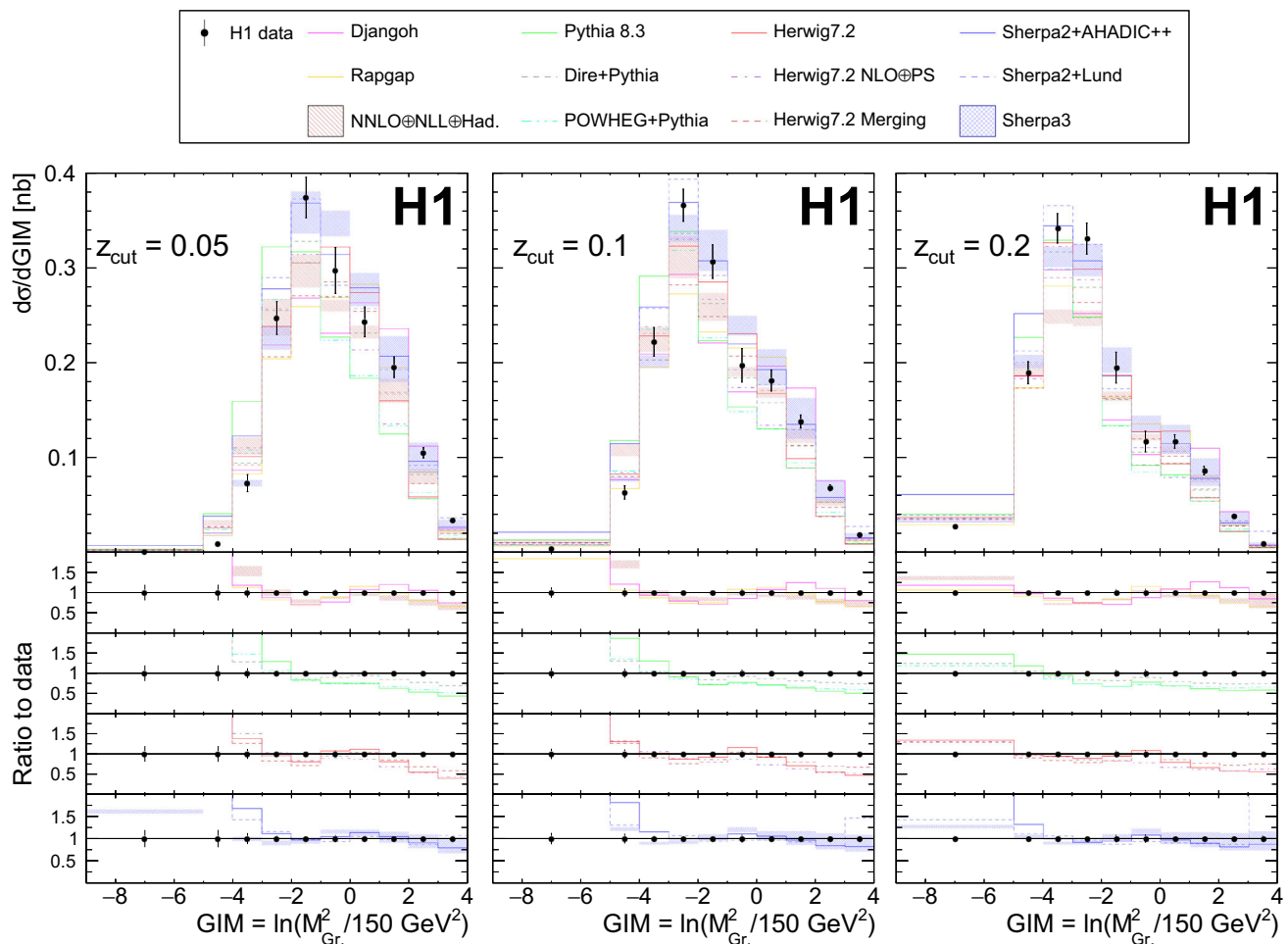
Fig. 2 Differential cross section of groomed invariant mass GIM = \ln(M_{Gr}^2/150 \text{ GeV}^2) in ep DIS at \sqrt{s} = 319 \text{ GeV} , for z_{cut} = 0.05 , 0.1 and, 0.2 . The value of Q_{min}^2 is set to 150 \text{ GeV}^2 . The phase space is restricted to Q^2 > 150 \text{ GeV}^2 and 0.2 < y < 0.7 . Uncertainty bars on
