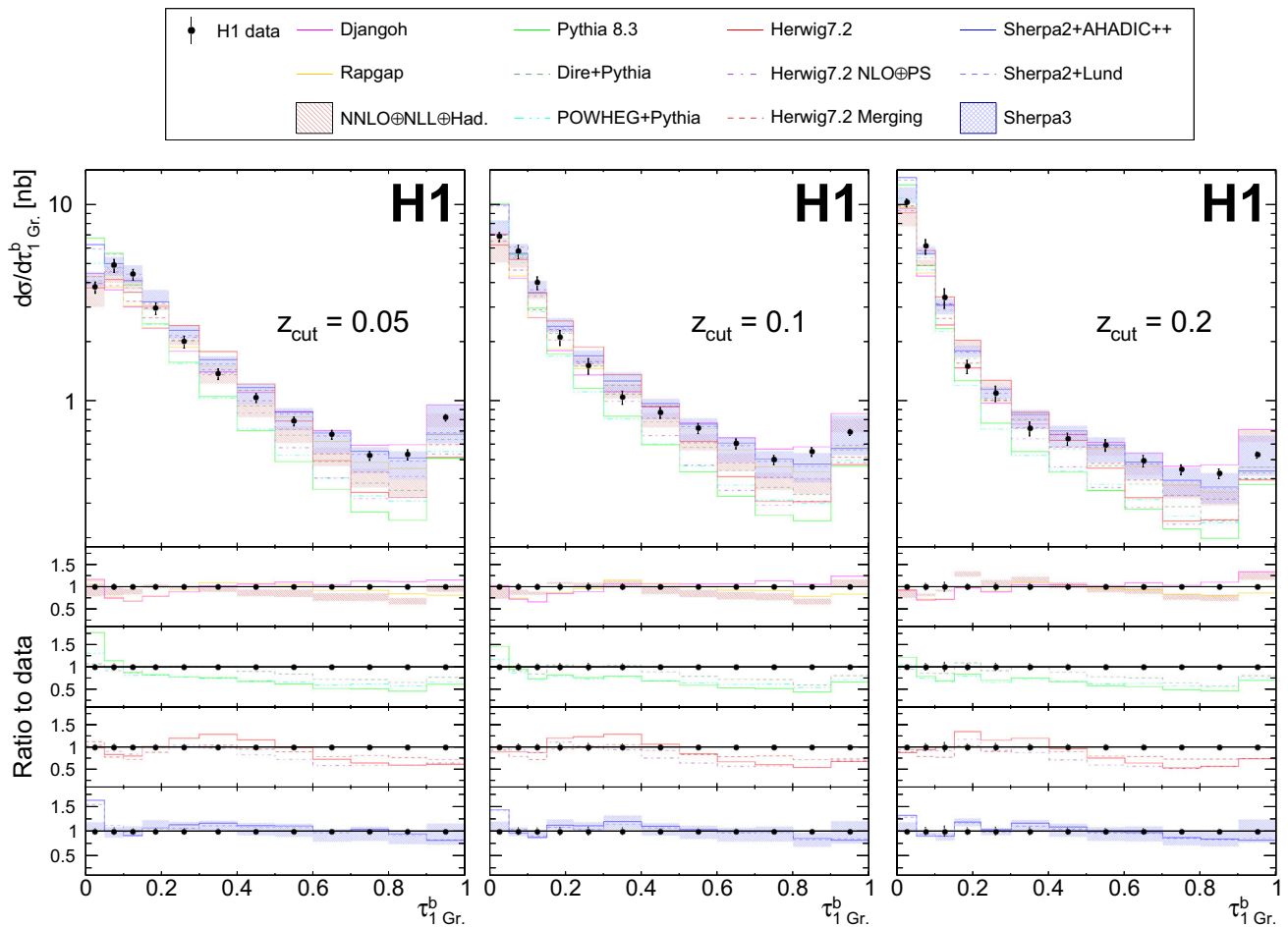
Fig. 3 Differential cross section of groomed 1-jettiness \tau_{1\text{Gr}}^b in ep DIS at \sqrt{s} = 319 GeV, for z_{\text{cut}} = 0.05, 0.1 and 0.2 . The phase space is restricted to Q^2 > 150 \text{ GeV}^2 and 0.2 < y < 0.7 . Uncertainty bars on
