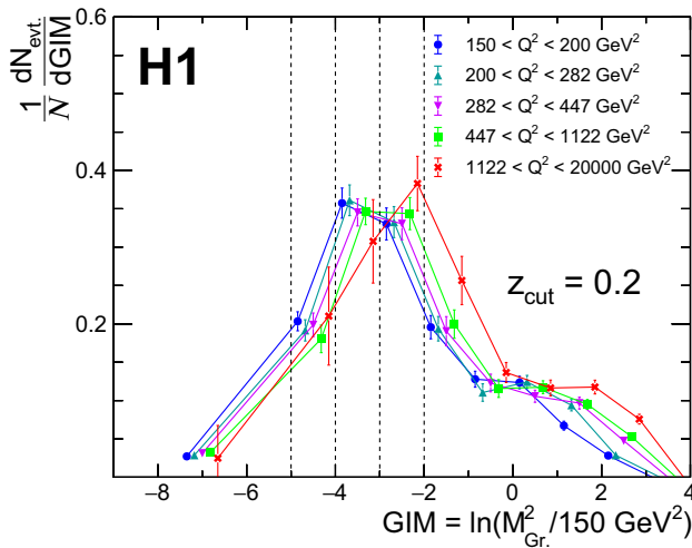
Fig. 5 Number of events as a function of GIM for z_{cut} = 0.2 in several Q^2 bins, with integral normalized to unity in the region GIM < -2 . Q_{min}^2 . Vertical dotted lines show bin boundaries of bins used in the normalization. The data points are offset horizontally for clarity. The bins have been scaled by their width
