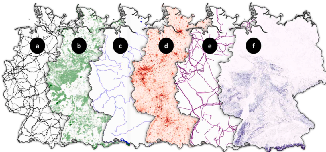
Fig. 2. Datasets used in the model. a) Main roads (dotted) and railways (hashed); b) CCDA areas (light green) and national parks (dark green); c) waterways and lakes; d) population density; e) pre-existing gas pipelines; f) terrain slope.
