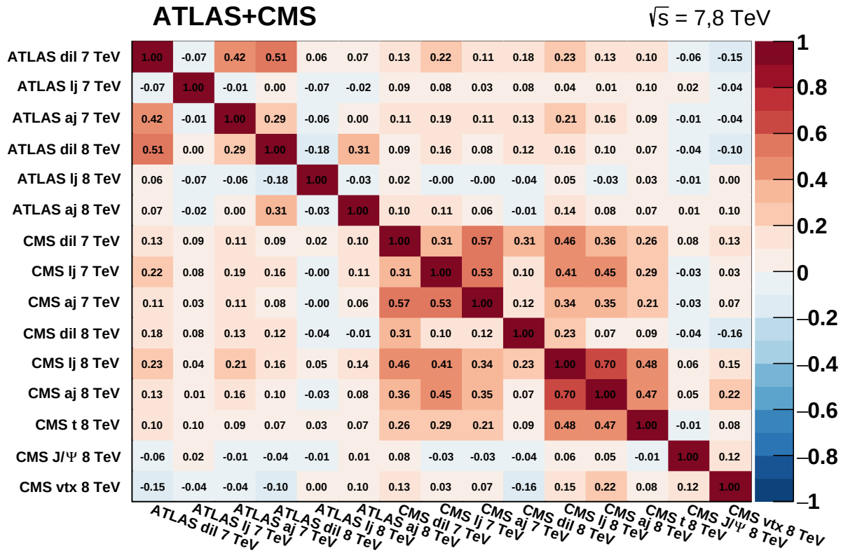
Figure A.2: Correlation matrix for the ATLAS and CMS 7 and 8 TeV m_t measurements in the dilepton (“dil”), lepton+jets (“lj”), and all-jets (“aj”) channels, and for the CMS 8 TeV m_t measurements in the single top (“t”), secondary vertex (“vtx”), and J/\psi analysis (“ J/\psi ”).
