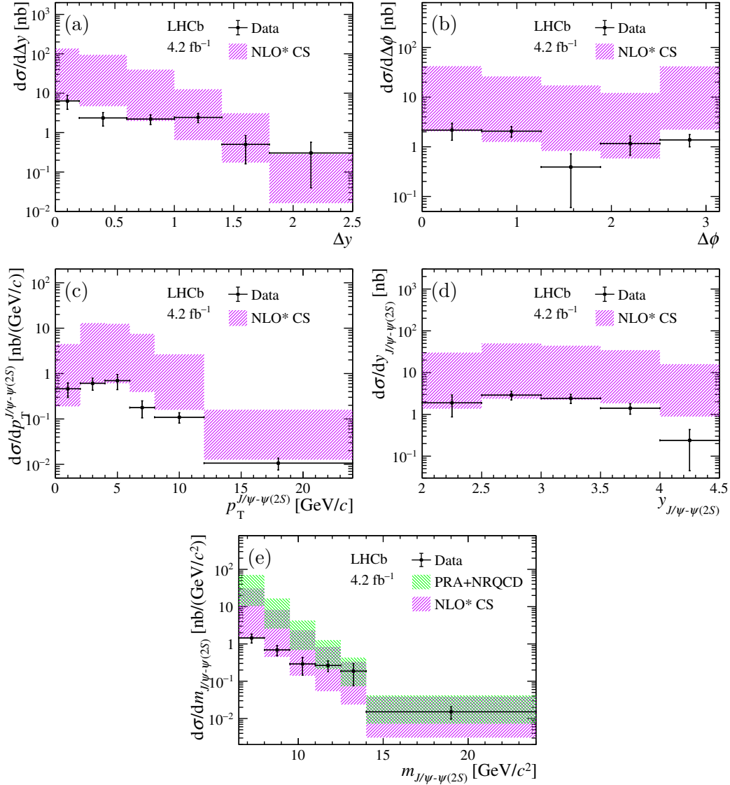
Figure 3. Differential cross-section of J/\psi - \psi(2S) production as a function of (a) \Delta y , (b) \Delta\phi , (c) p_T^{J/\psi-\psi(2S)} , (d) y_{J/\psi-\psi(2S)} and (e) m_{J/\psi-\psi(2S)} , compared with the NLO* CS predictions for SPS [54–56]. The m_{J/\psi-\psi(2S)} spectrum is also compared with the PRA+NRQCD predictions for SPS [57]. The data contain contributions from both SPS and DPS.
