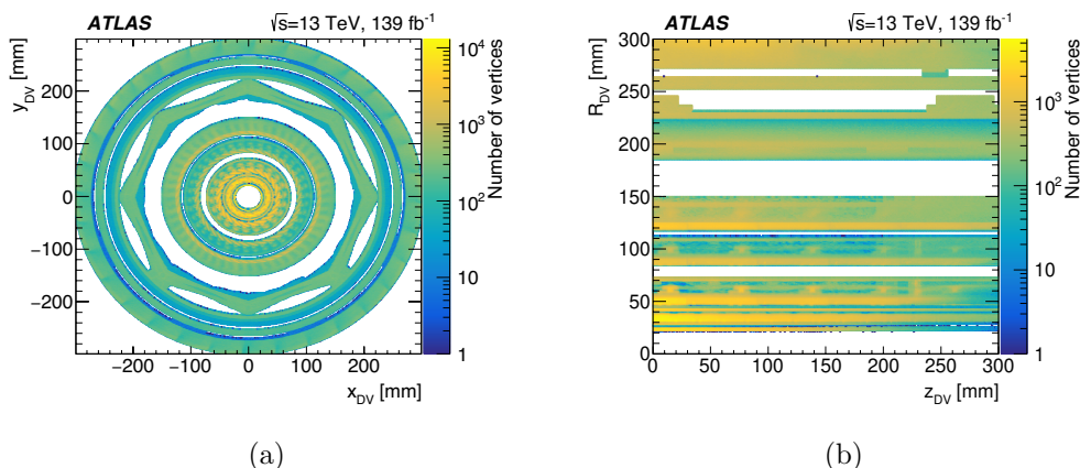
Figure 3. The positions in the (a) x-y plane and (b) r-z plane of reconstructed displaced vertices that are vetoed by the material map in the analyzed data sample. The right figure is restricted to positive z values for presentation. The innermost area corresponds to the beampipe. This is surrounded by four pixel detector layers. The octagonal shape and outermost structures are due to support structures separating the pixel and SCT detectors.
