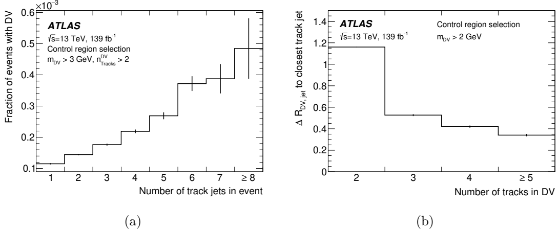
Figure 4. In (a), the fraction of events in the CR with a reconstructed DV satisfying m_{\text{DV}} > 3 \text{ GeV} and n_{\text{Tracks}}^{\text{DV}} > 2 is shown. In (b), the average distance of DVs with m_{\text{DV}} > 2 \text{ GeV} to the closest track jet in the event is shown, as a function of n_{\text{Tracks}} .
