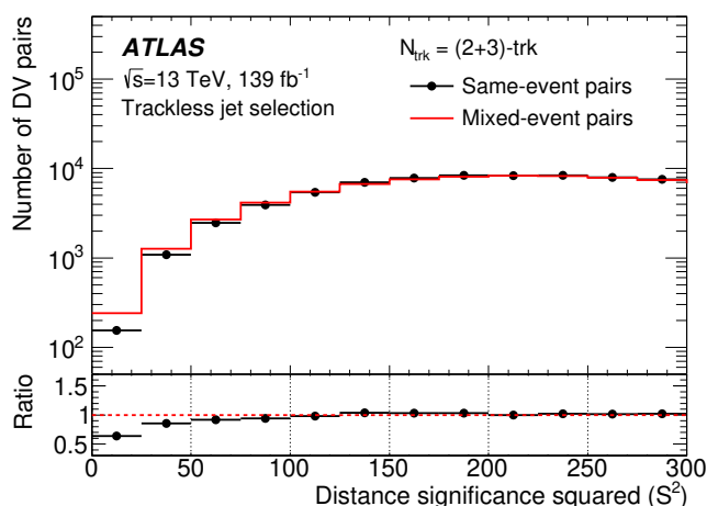
Figure 6. Squared significance of the distance between pairs of preselected DVs with two and three tracks (denoted by n_{\text{Tracks}}^{\text{DV}} = (2+3)\text{-trk} ) taken from the same event and from distinct events passing the Trackless jet selection. The mixed event distribution is normalized to match the same event distribution in the S^2 > 100 region.
