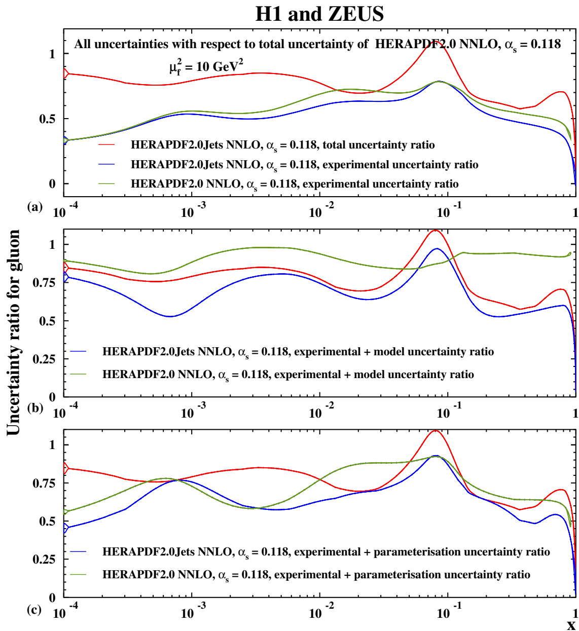
Fig. 23 Ratios of uncertainties relative to the total uncertainties of HERAPDF2.0 NNLO with \alpha_s(M_Z^2) = 0.118 for the total uncertainty of HERAPDF2.0Jets NNLO with \alpha_s(M_Z^2) = 0.118 and the a experimental, b experimental plus model, c experimental plus parameteri-
