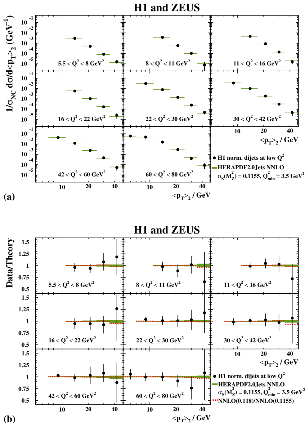
Fig. 16 a Differential dijet-cross-section predictions, d\sigma/d\langle p_T \rangle_2 , based on HERAPDF2.0Jets NNLO with \alpha_s(M_Z^2) = 0.1155 in bins of Q^2 between 5.5 and 80 \text{GeV}^2 compared to H1 data normalised to neutral current (NC) inclusive cross sections [14]. The variable \langle p_T \rangle_2 denotes the average p_T of the two jets. Only data used in the fit are shown. b Measured dijet cross sections divided by predictions based
