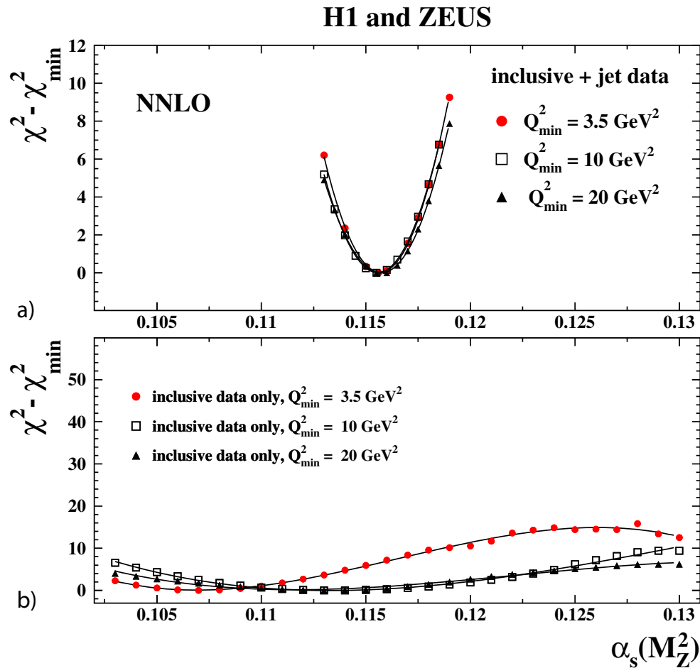
Fig. 3 Difference between \chi^2 and \chi_{\min}^2 versus \alpha_s(M_Z^2) for a HERAPDF2.0Jets NNLO fits with fixed \alpha_s(M_Z^2) with the standard Q_{\min}^2 for the inclusive data of 3.5 GeV 2 and Q_{\min}^2 set to
